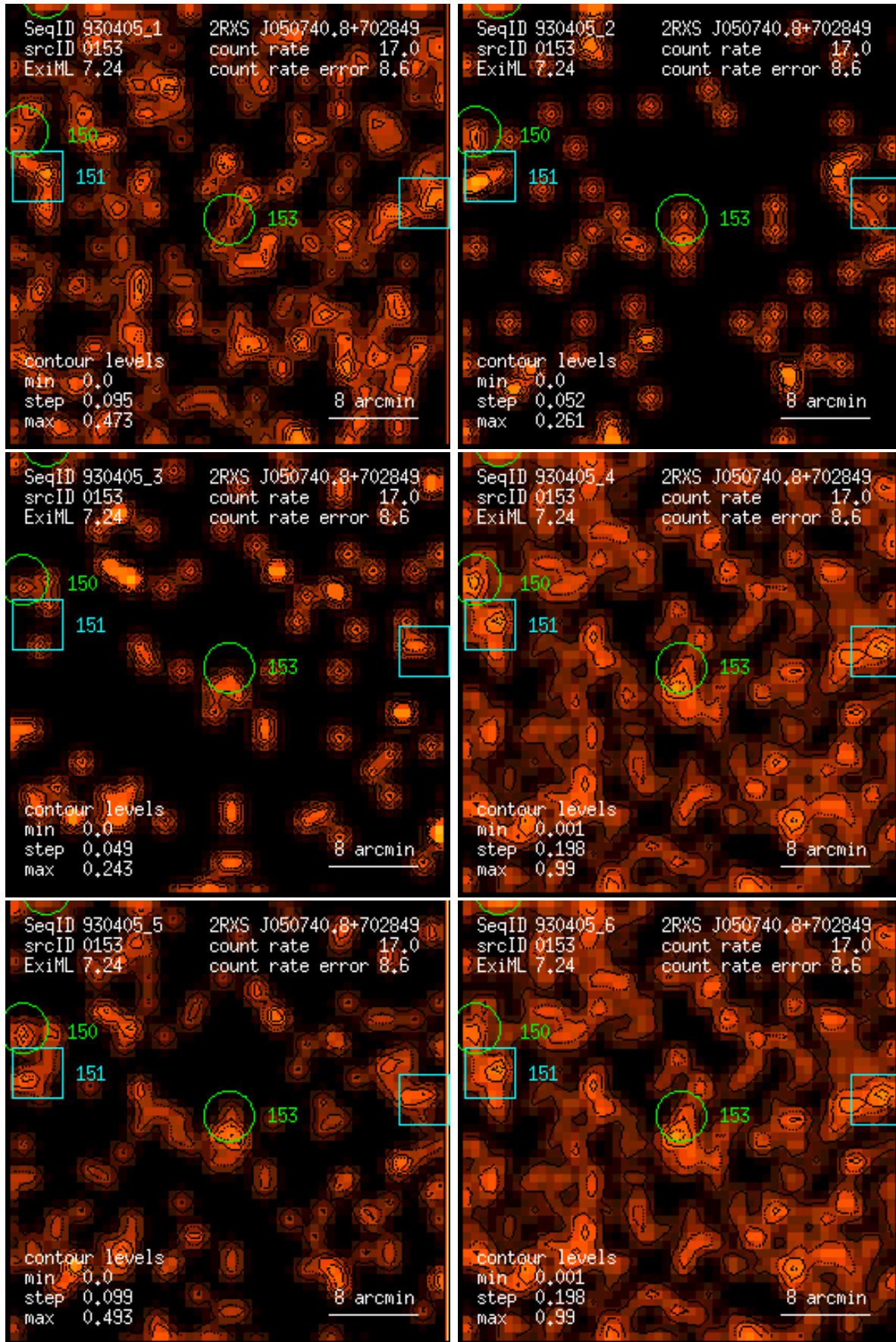
Figure 153: RASS 930405: detection 0153: band rate images, Gaussian filter: (1) PSPC channels 11 – 41, (2) 52 – 90, (3) 91 – 201, (4) 11 – 235, (5) 52 – 201, (6) 11 – 201. Broad band rates in counts/ks. Band rate contour levels in counts/ks/arcmin 2 .
