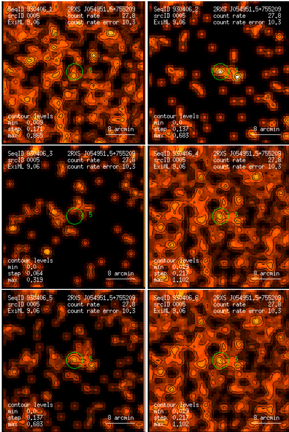
Figure 5: RASS 930406: detection 0005: band rate images, Gaussian filter: (1) PSPC channels 11 – 41, (2) 52 – 90, (3) 91 – 201, (4) 11 – 235, (5) 52 – 201, (6) 11 – 201. Broad band rates in counts/ks. Band rate contour levels in counts/ks/arcmin 2 .
