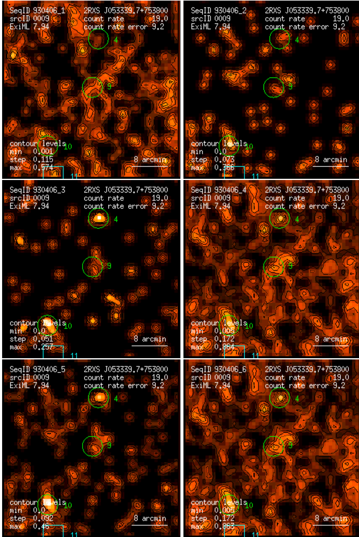
Figure 9: RASS 930406: detection 0009: band rate images, Gaussian filter: (1) PSPC channels 11 – 41, (2) 52 – 90, (3) 91 – 201, (4) 11 – 235, (5) 52 – 201, (6) 11 – 201. Broad band rates in counts/ks. Band rate contour levels in counts/ks/arcmin 2 .
