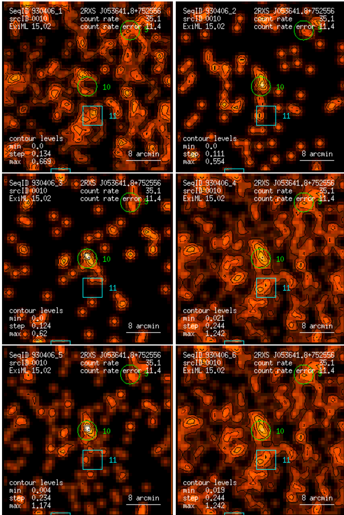
Figure 10: RASS 930406: detection 0010: band rate images, Gaussian filter: (1) PSPC channels 11 – 41, (2) 52 – 90, (3) 91 – 201, (4) 11 – 235, (5) 52 – 201, (6) 11 – 201. Broad band rates in counts/ks. Band rate contour levels in counts/ks/arcmin 2 .
