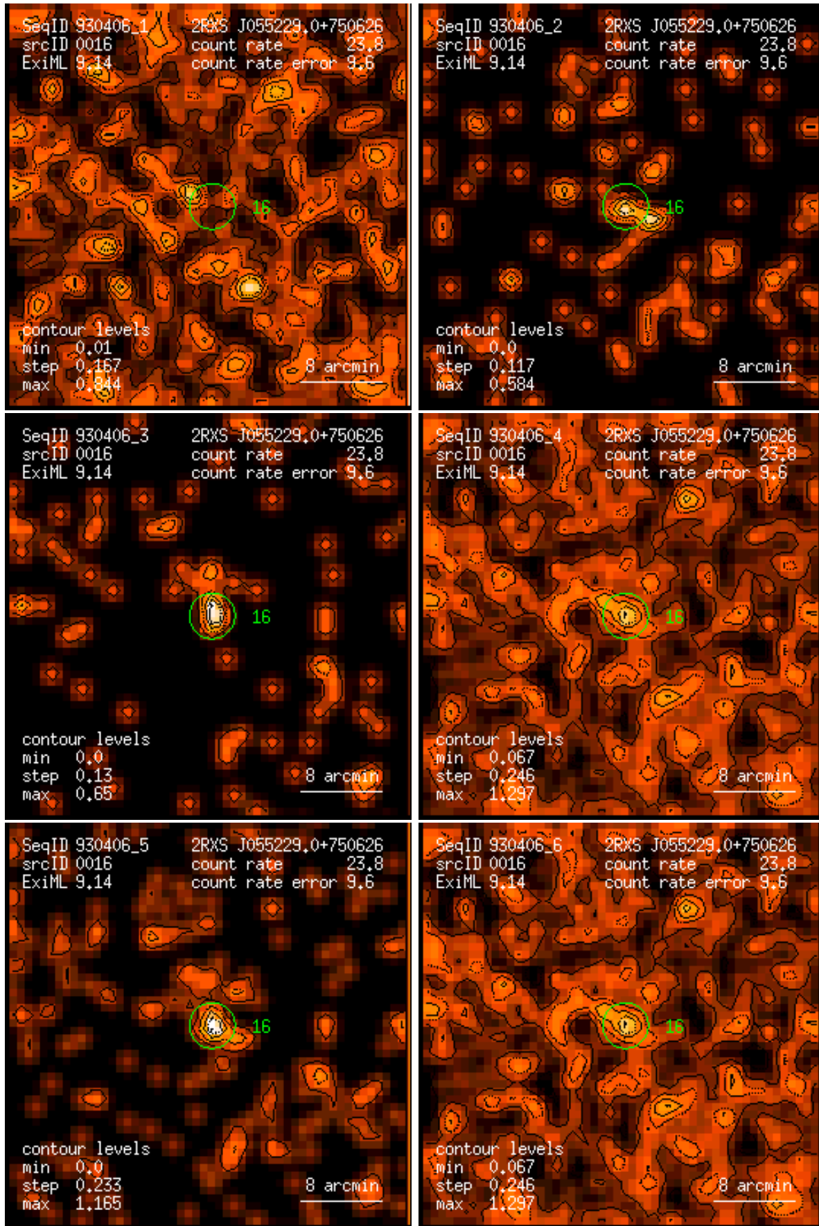
Figure 16: RASS 930406: detection 0016: band rate images, Gaussian filter: (1) PSPC channels 11 – 41, (2) 52 – 90, (3) 91 – 201, (4) 11 – 235, (5) 52 – 201, (6) 11 – 201. Broad band rates in counts/ks. Band rate contour levels in counts/ks/arcmin 2 .
