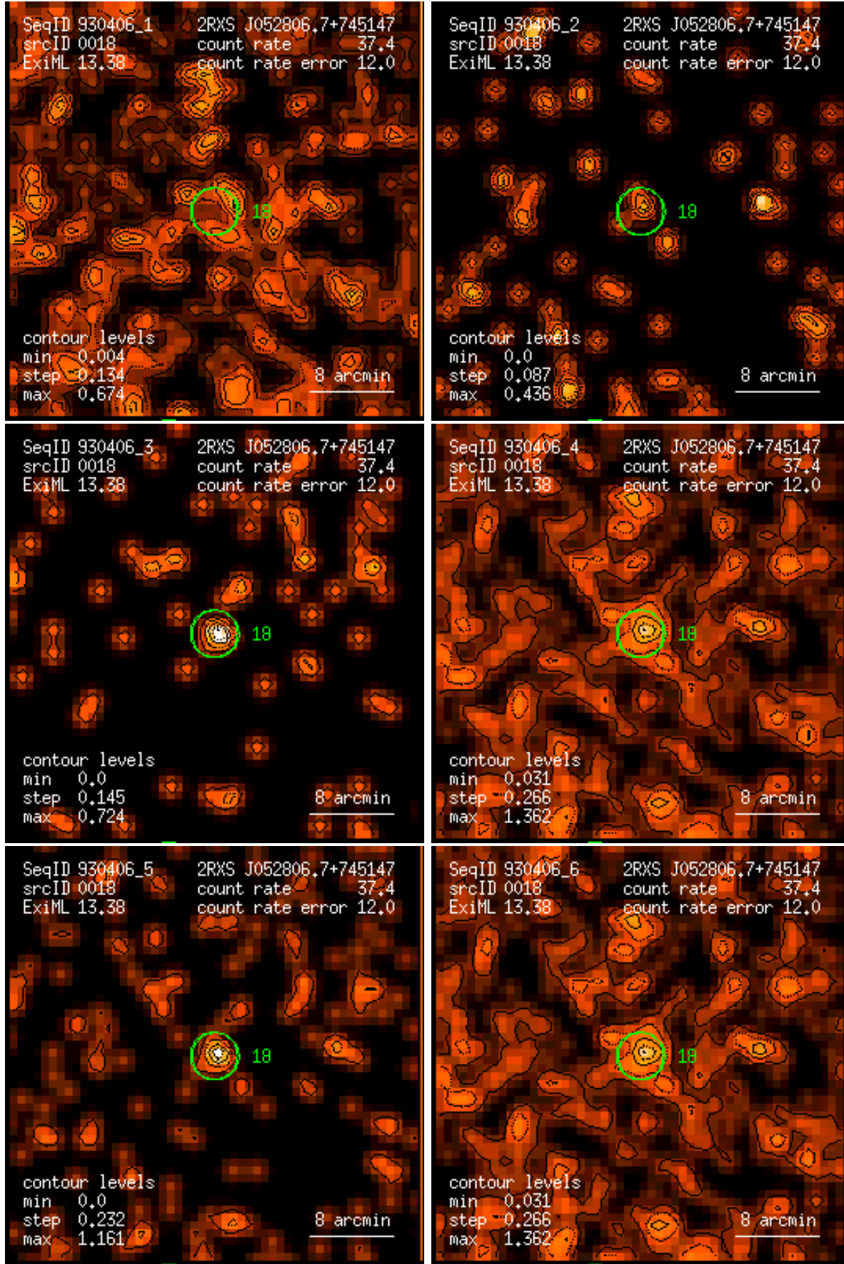
Figure 18: RASS 930406: detection 0018: band rate images, Gaussian filter: (1) PSPC channels 11 – 41, (2) 52 – 90, (3) 91 – 201, (4) 11 – 235, (5) 52 – 201, (6) 11 – 201. Broad band rates in counts/ks. Band rate contour levels in counts/ks/arcmin 2 .
