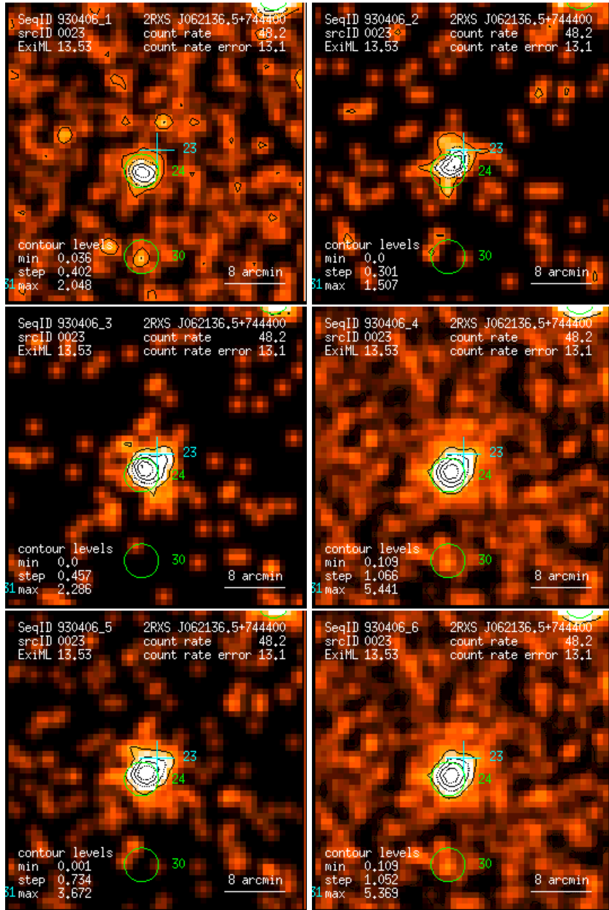
Figure 23: RASS 930406: detection 0023: band rate images, Gaussian filter: (1) PSPC channels 11 – 41, (2) 52 – 90, (3) 91 – 201, (4) 11 – 235, (5) 52 – 201, (6) 11 – 201. Broad band rates in counts/ks. Band rate contour levels in counts/ks/arcmin 2 .
