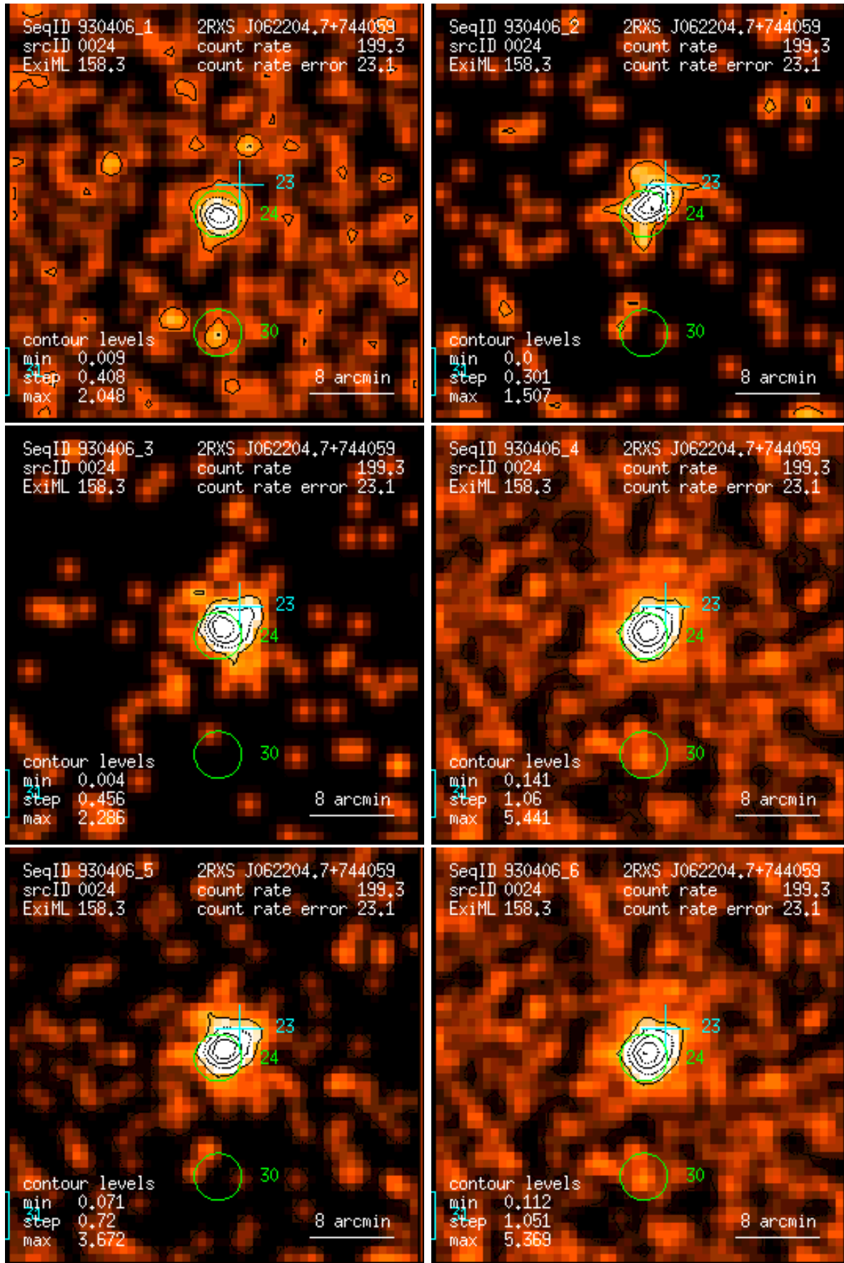
Figure 24: RASS 930406: detection 0024: band rate images, Gaussian filter: (1) PSPC channels 11 – 41, (2) 52 – 90, (3) 91 – 201, (4) 11 – 235, (5) 52 – 201, (6) 11 – 201. Broad band rates in counts/ks. Band rate contour levels in counts/ks/arcmin 2 .
