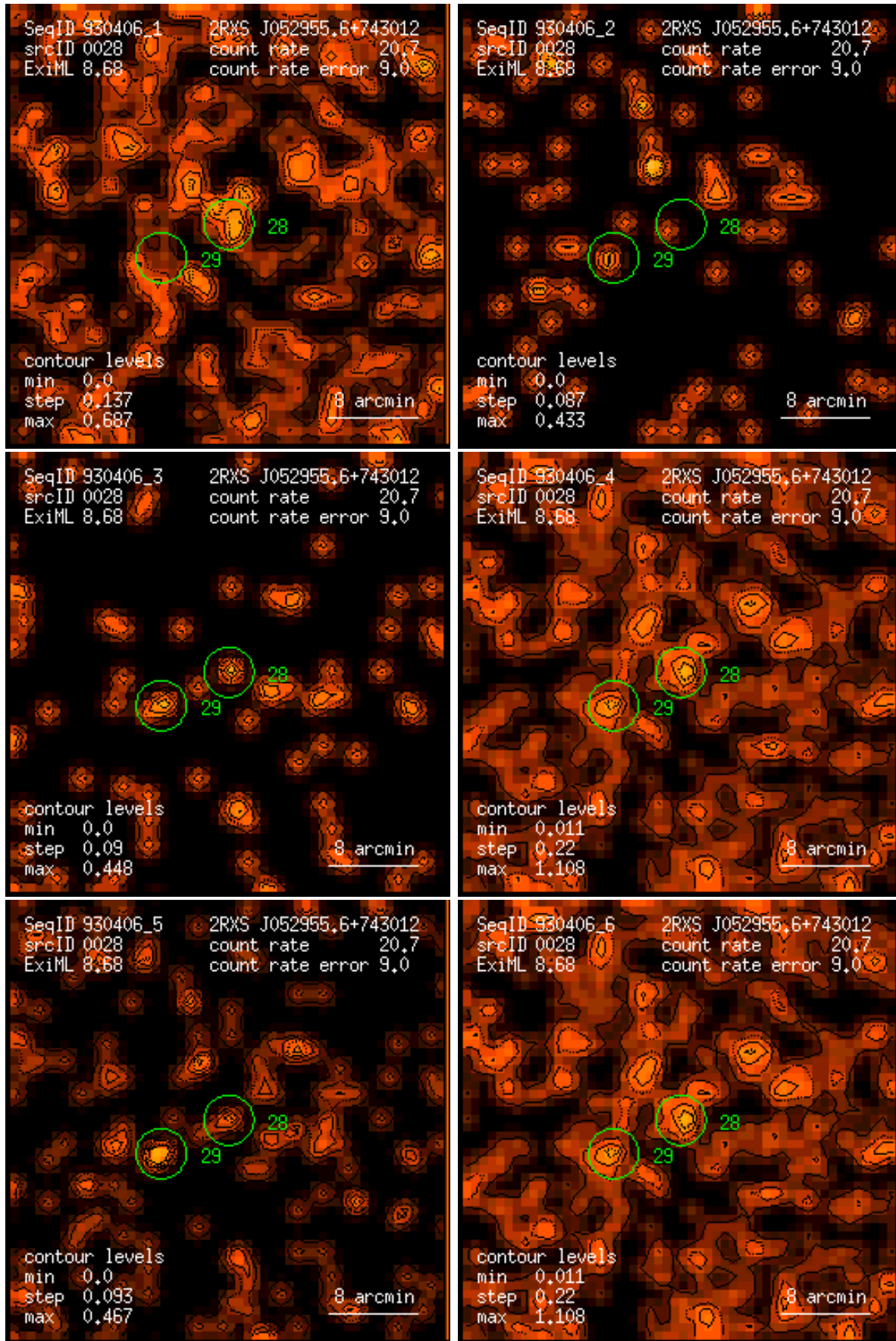
Figure 28: RASS 930406: detection 0028: band rate images, Gaussian filter: (1) PSPC channels 11 – 41, (2) 52 – 90, (3) 91 – 201, (4) 11 – 235, (5) 52 – 201, (6) 11 – 201. Broad band rates in counts/ks. Band rate contour levels in counts/ks/arcmin 2 .
