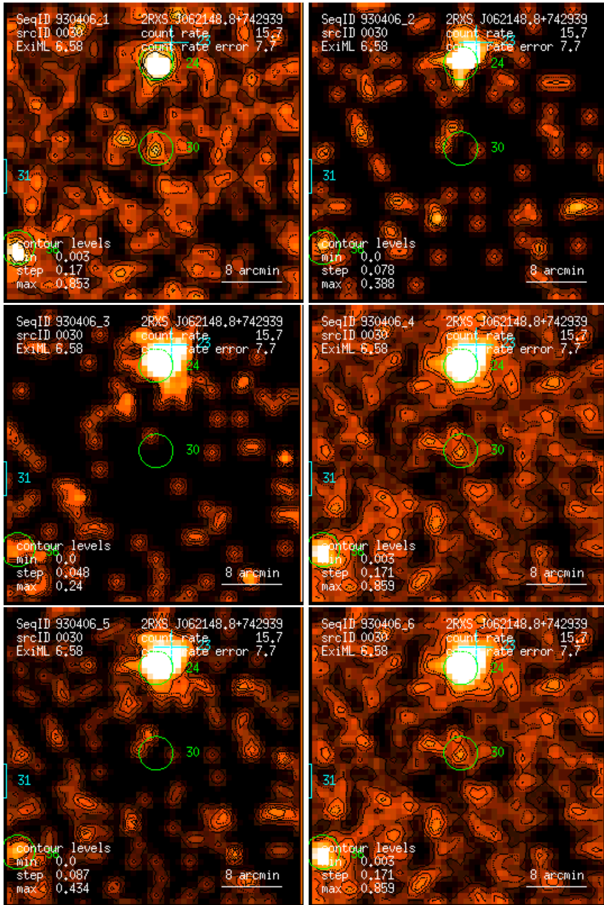
Figure 30: RASS 930406: detection 0030: band rate images, Gaussian filter: (1) PSPC channels 11 – 41, (2) 52 – 90, (3) 91 – 201, (4) 11 – 235, (5) 52 – 201, (6) 11 – 201. Broad band rates in counts/ks. Band rate contour levels in counts/ks/arcmin 2 .
