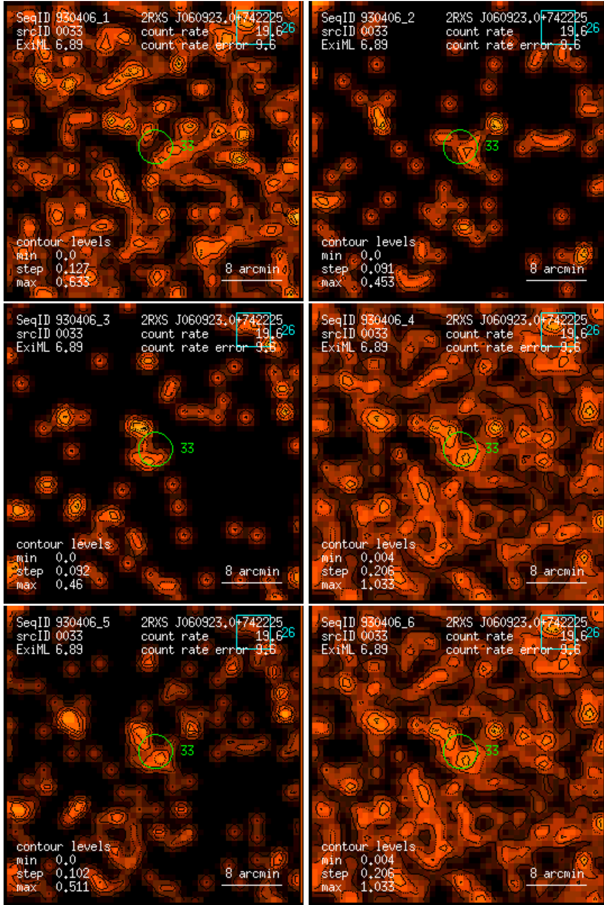
Figure 33: RASS 930406: detection 0033: band rate images, Gaussian filter: (1) PSPC channels 11 – 41, (2) 52 – 90, (3) 91 – 201, (4) 11 – 235, (5) 52 – 201, (6) 11 – 201. Broad band rates in counts/ks. Band rate contour levels in counts/ks/arcmin 2 .
