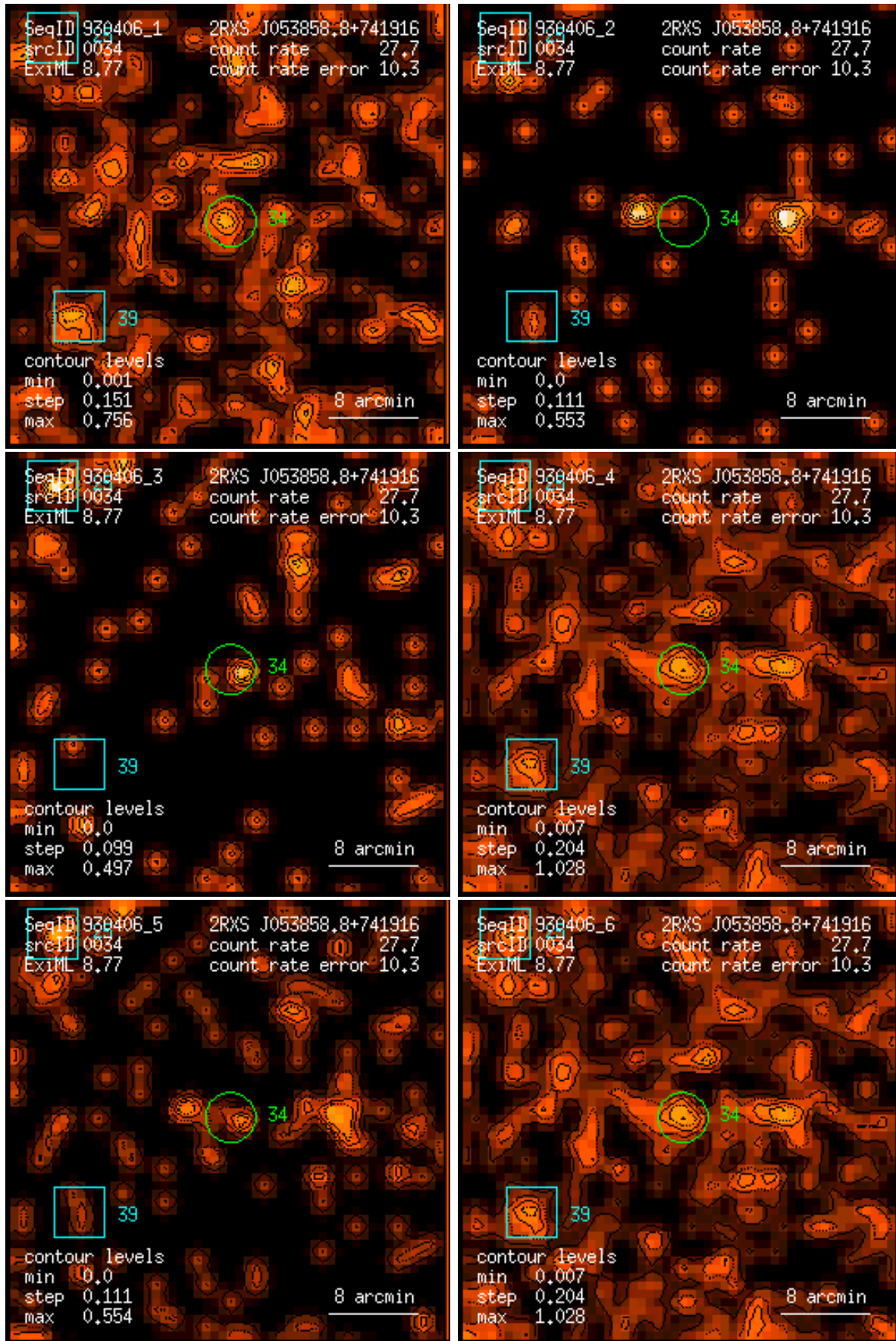
Figure 34: RASS 930406: detection 0034: band rate images, Gaussian filter: (1) PSPC channels 11 – 41, (2) 52 – 90, (3) 91 – 201, (4) 11 – 235, (5) 52 – 201, (6) 11 – 201. Broad band rates in counts/ks. Band rate contour levels in counts/ks/arcmin 2 .
