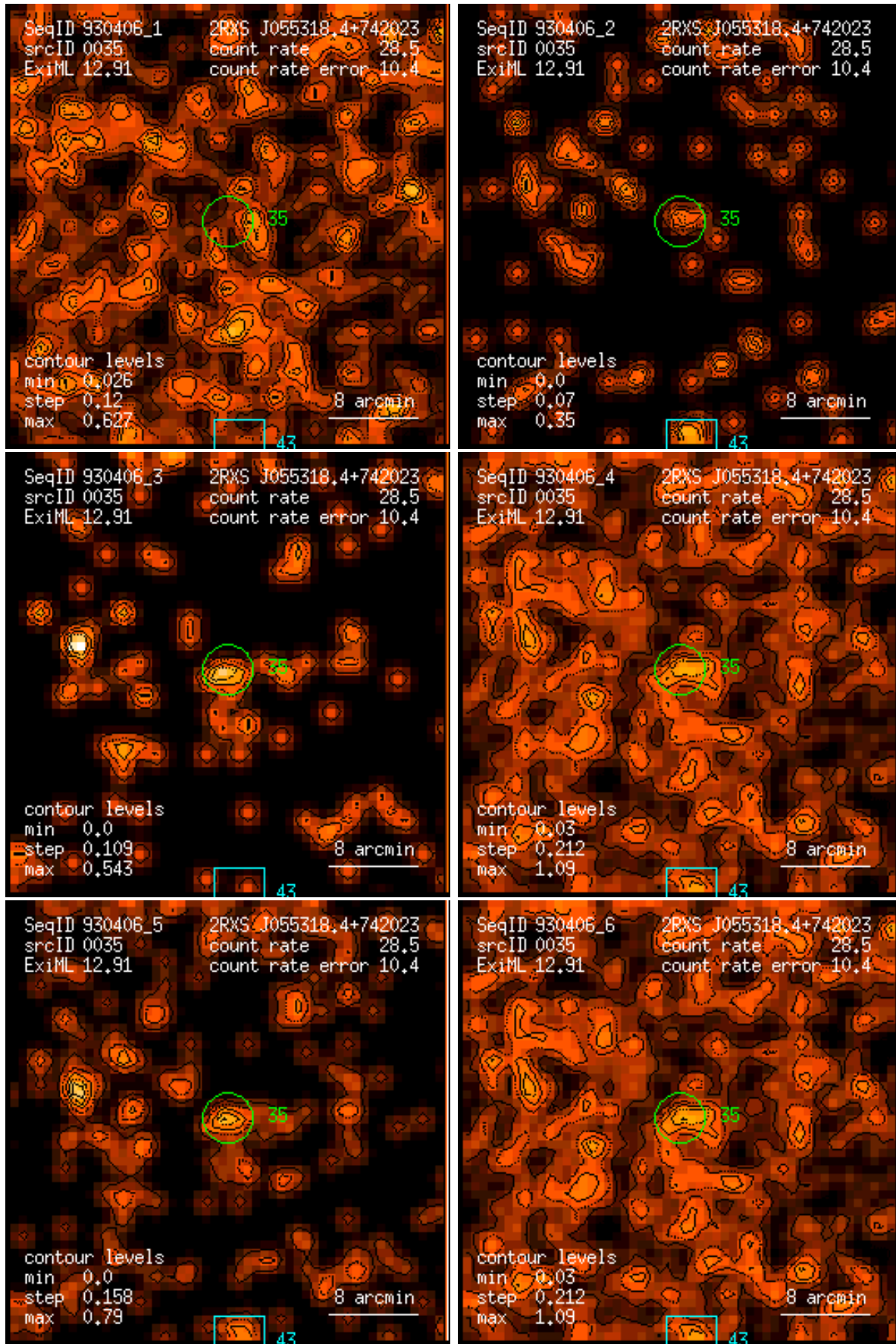
Figure 35: RASS 930406: detection 0035: band rate images, Gaussian filter: (1) PSPC channels 11 – 41, (2) 52 – 90, (3) 91 – 201, (4) 11 – 235, (5) 52 – 201, (6) 11 – 201. Broad band rates in counts/ks. Band rate contour levels in counts/ks/arcmin 2 .
