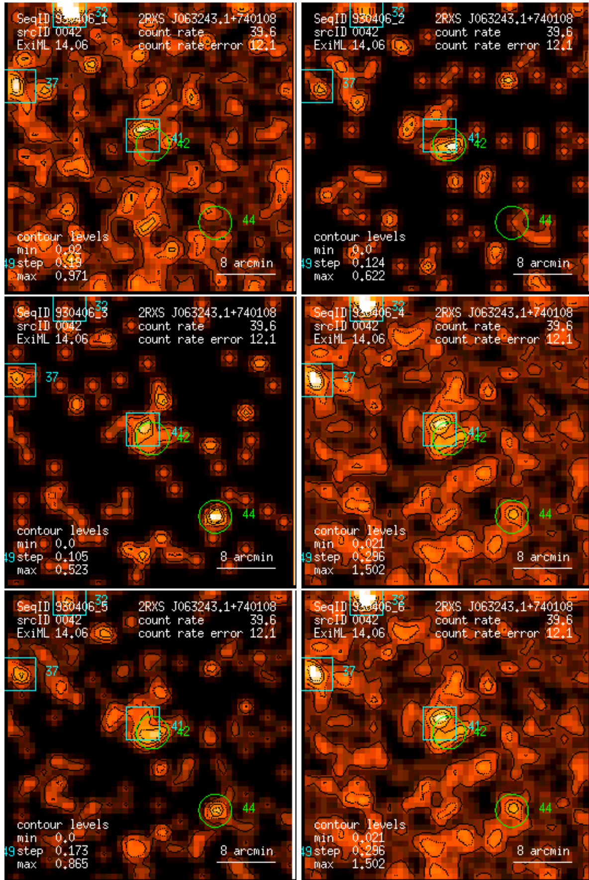
Figure 42: RASS 930406: detection 0042: band rate images, Gaussian filter: (1) PSPC channels 11 – 41, (2) 52 – 90, (3) 91 – 201, (4) 11 – 235, (5) 52 – 201, (6) 11 – 201. Broad band rates in counts/ks. Band rate contour levels in counts/ks/arcmin 2 .
