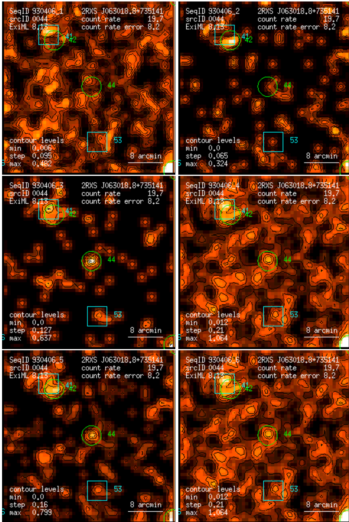
Figure 44: RASS 930406: detection 0044: band rate images, Gaussian filter: (1) PSPC channels 11 – 41, (2) 52 – 90, (3) 91 – 201, (4) 11 – 235, (5) 52 – 201, (6) 11 – 201. Broad band rates in counts/ks. Band rate contour levels in counts/ks/arcmin 2 .
