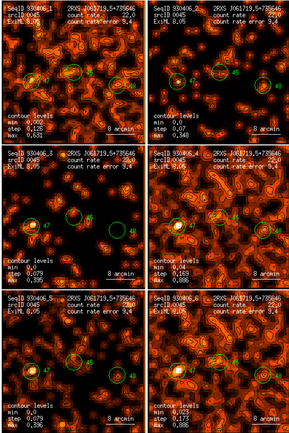
Figure 45: RASS 930406: detection 0045: band rate images, Gaussian filter: (1) PSPC channels 11 – 41, (2) 52 – 90, (3) 91 – 201, (4) 11 – 235, (5) 52 – 201, (6) 11 – 201. Broad band rates in counts/ks. Band rate contour levels in counts/ks/arcmin 2 .
