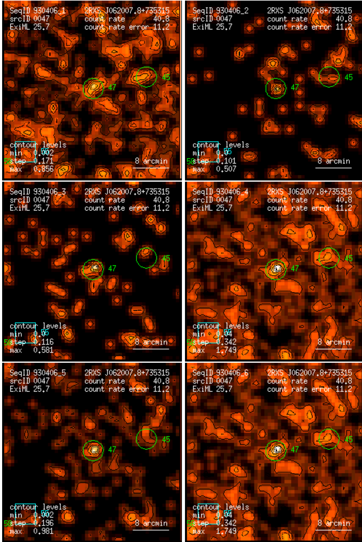
Figure 47: RASS 930406: detection 0047: band rate images, Gaussian filter: (1) PSPC channels 11 – 41, (2) 52 – 90, (3) 91 – 201, (4) 11 – 235, (5) 52 – 201, (6) 11 – 201. Broad band rates in counts/ks. Band rate contour levels in counts/ks/arcmin 2 .
