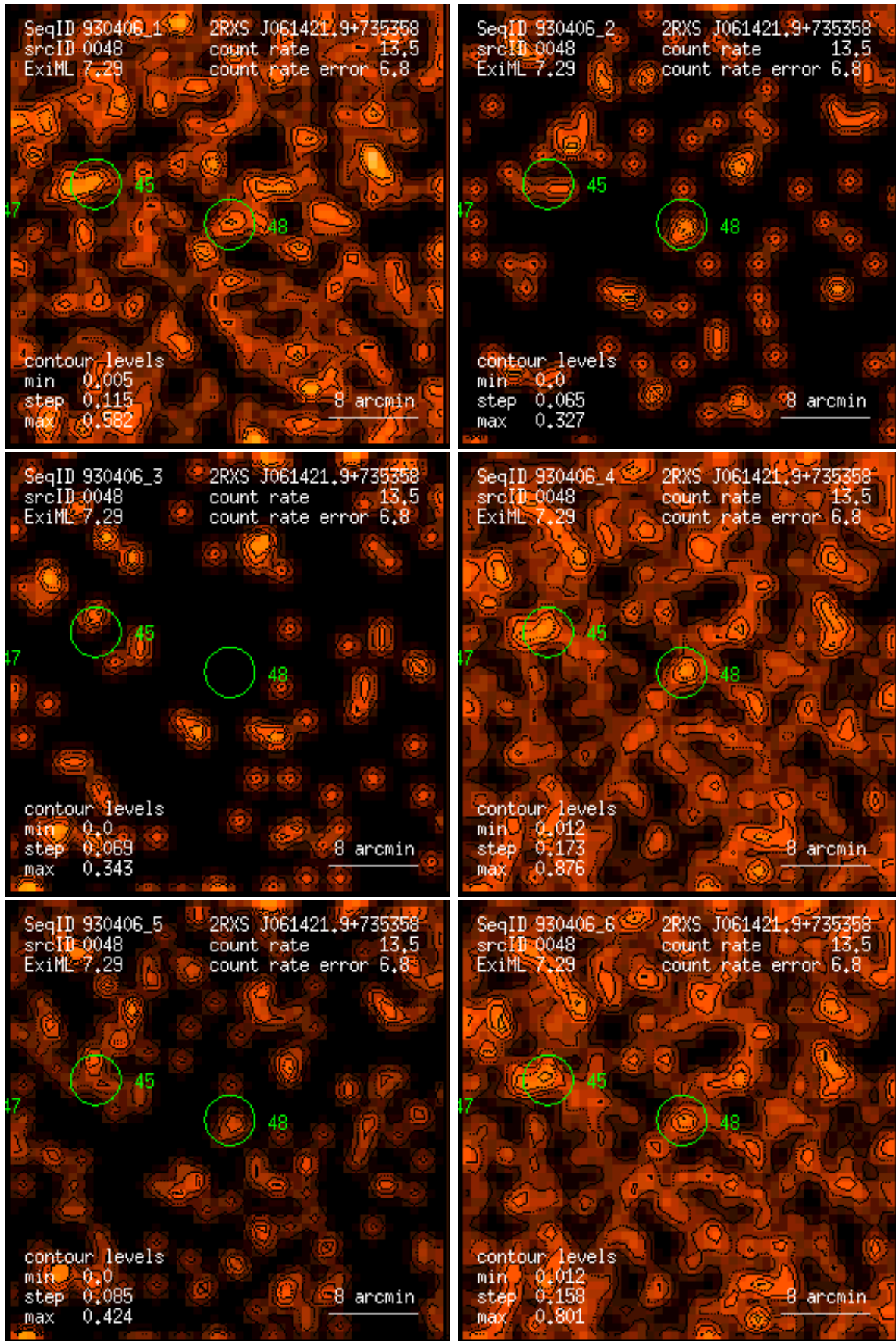
Figure 48: RASS 930406: detection 0048: band rate images, Gaussian filter: (1) PSPC channels 11 – 41, (2) 52 – 90, (3) 91 – 201, (4) 11 – 235, (5) 52 – 201, (6) 11 – 201. Broad band rates in counts/ks. Band rate contour levels in counts/ks/arcmin 2 .
