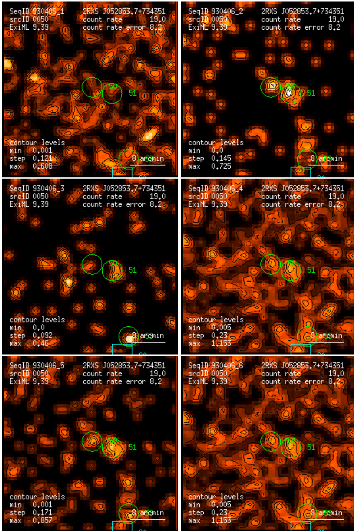
Figure 50: RASS 930406: detection 0050: band rate images, Gaussian filter: (1) PSPC channels 11 – 41, (2) 52 – 90, (3) 91 – 201, (4) 11 – 235, (5) 52 – 201, (6) 11 – 201. Broad band rates in counts/ks. Band rate contour levels in counts/ks/arcmin 2 .
