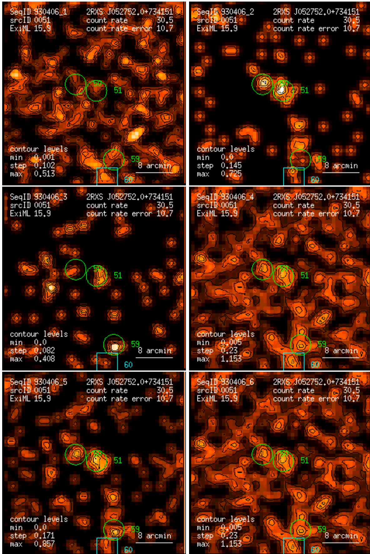
Figure 51: RASS 930406: detection 0051: band rate images, Gaussian filter: (1) PSPC channels 11 – 41, (2) 52 – 90, (3) 91 – 201, (4) 11 – 235, (5) 52 – 201, (6) 11 – 201. Broad band rates in counts/ks. Band rate contour levels in counts/ks/arcmin 2 .
