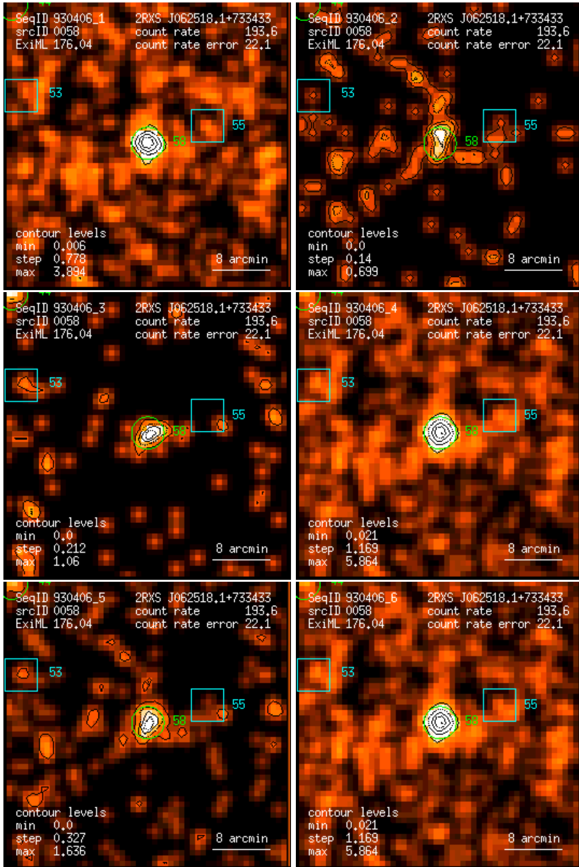
Figure 58: RASS 930406: detection 0058: band rate images, Gaussian filter: (1) PSPC channels 11 – 41, (2) 52 – 90, (3) 91 – 201, (4) 11 – 235, (5) 52 – 201, (6) 11 – 201. Broad band rates in counts/ks. Band rate contour levels in counts/ks/arcmin 2 .
