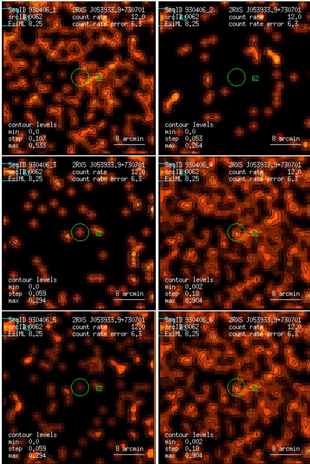
Figure 62: RASS 930406: detection 0062: band rate images, Gaussian filter: (1) PSPC channels 11 – 41, (2) 52 – 90, (3) 91 – 201, (4) 11 – 235, (5) 52 – 201, (6) 11 – 201. Broad band rates in counts/ks. Band rate contour levels in counts/ks/arcmin 2 .
