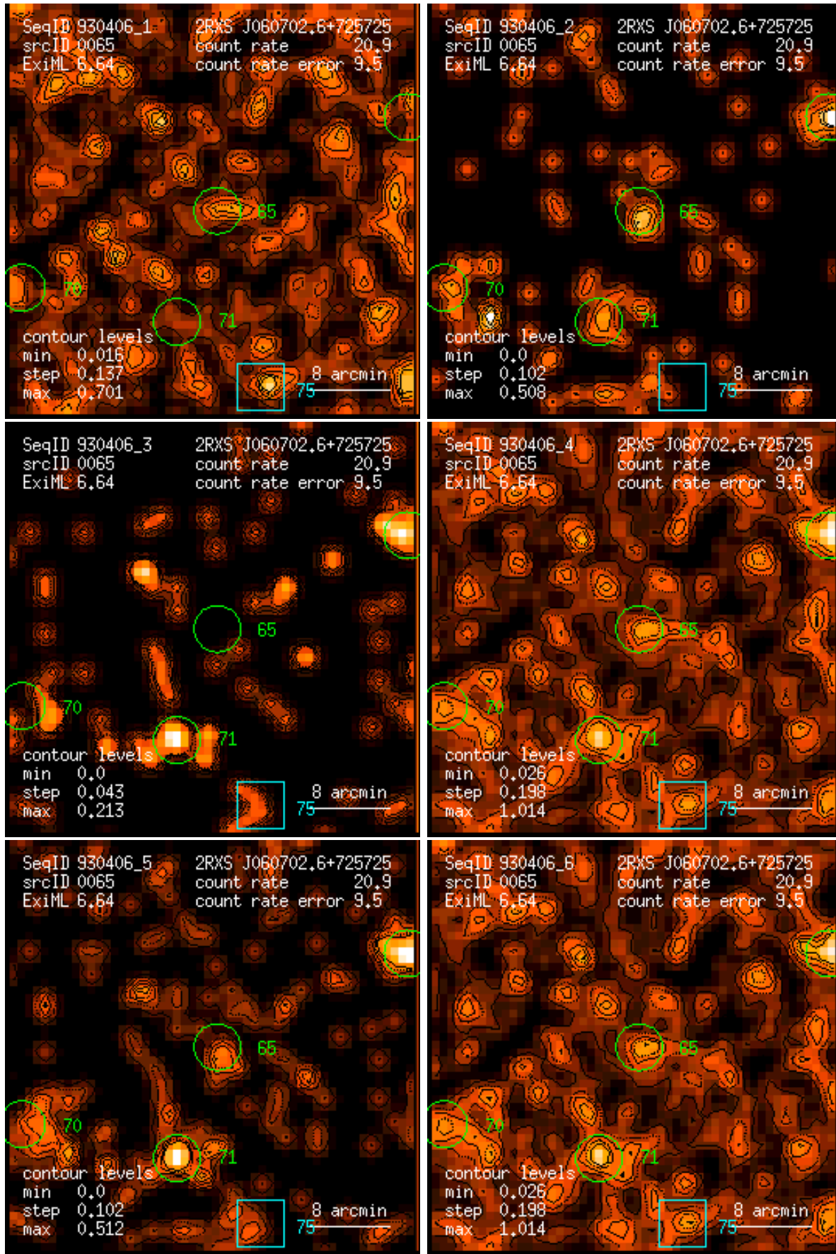
Figure 65: RASS 930406: detection 0065: band rate images, Gaussian filter: (1) PSPC channels 11 – 41, (2) 52 – 90, (3) 91 – 201, (4) 11 – 235, (5) 52 – 201, (6) 11 – 201. Broad band rates in counts/ks. Band rate contour levels in counts/ks/arcmin 2 .
