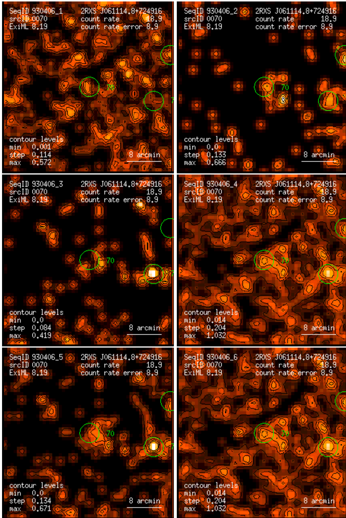
Figure 70: RASS 930406: detection 0070: band rate images, Gaussian filter: (1) PSPC channels 11 – 41, (2) 52 – 90, (3) 91 – 201, (4) 11 – 235, (5) 52 – 201, (6) 11 – 201. Broad band rates in counts/ks. Band rate contour levels in counts/ks/arcmin 2 .
