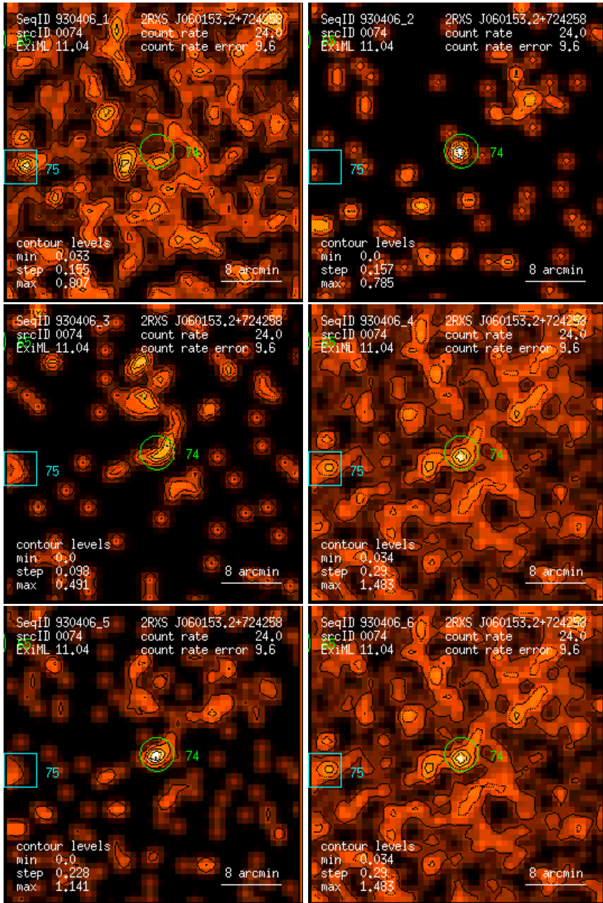
Figure 74: RASS 930406: detection 0074: band rate images, Gaussian filter: (1) PSPC channels 11 – 41, (2) 52 – 90, (3) 91 – 201, (4) 11 – 235, (5) 52 – 201, (6) 11 – 201. Broad band rates in counts/ks. Band rate contour levels in counts/ks/arcmin 2 .
