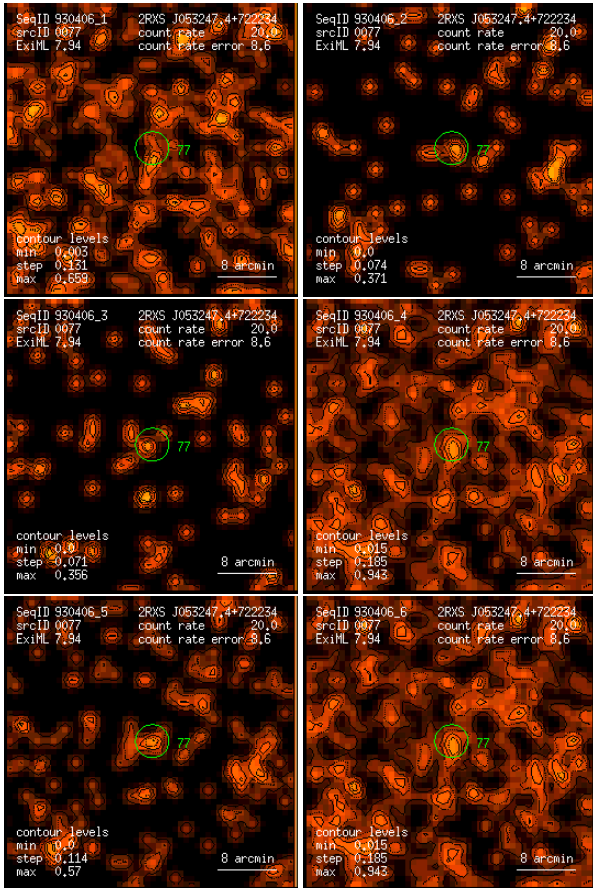
Figure 77: RASS 930406: detection 0077: band rate images, Gaussian filter: (1) PSPC channels 11 – 41, (2) 52 – 90, (3) 91 – 201, (4) 11 – 235, (5) 52 – 201, (6) 11 – 201. Broad band rates in counts/ks. Band rate contour levels in counts/ks/arcmin 2 .
