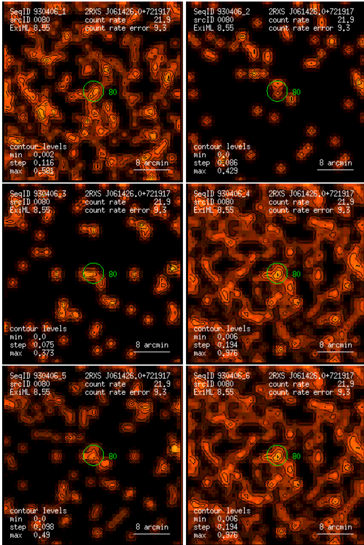
Figure 80: RASS 930406: detection 0080: band rate images, Gaussian filter: (1) PSPC channels 11 – 41, (2) 52 – 90, (3) 91 – 201, (4) 11 – 235, (5) 52 – 201, (6) 11 – 201. Broad band rates in counts/ks. Band rate contour levels in counts/ks/arcmin 2 .
