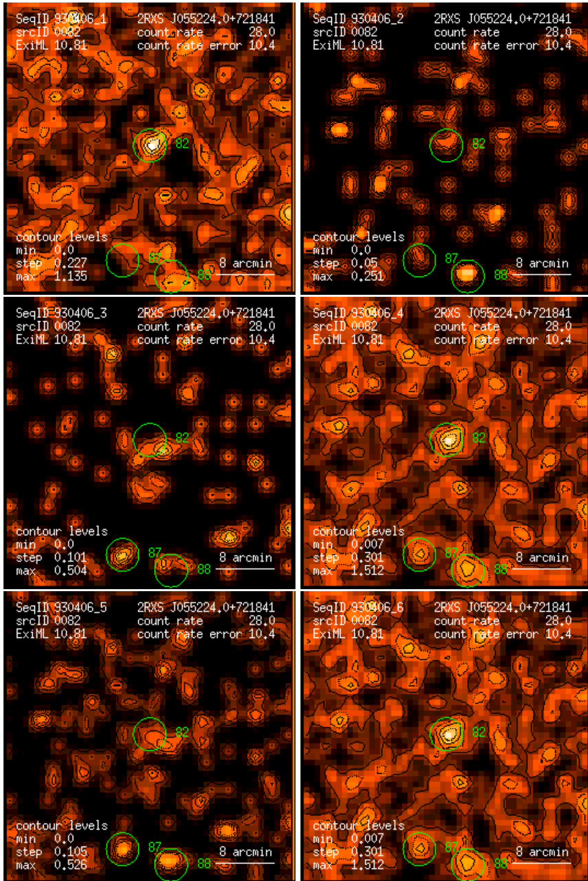
Figure 82: RASS 930406: detection 0082: band rate images, Gaussian filter: (1) PSPC channels 11 – 41, (2) 52 – 90, (3) 91 – 201, (4) 11 – 235, (5) 52 – 201, (6) 11 – 201. Broad band rates in counts/ks. Band rate contour levels in counts/ks/arcmin 2 .
