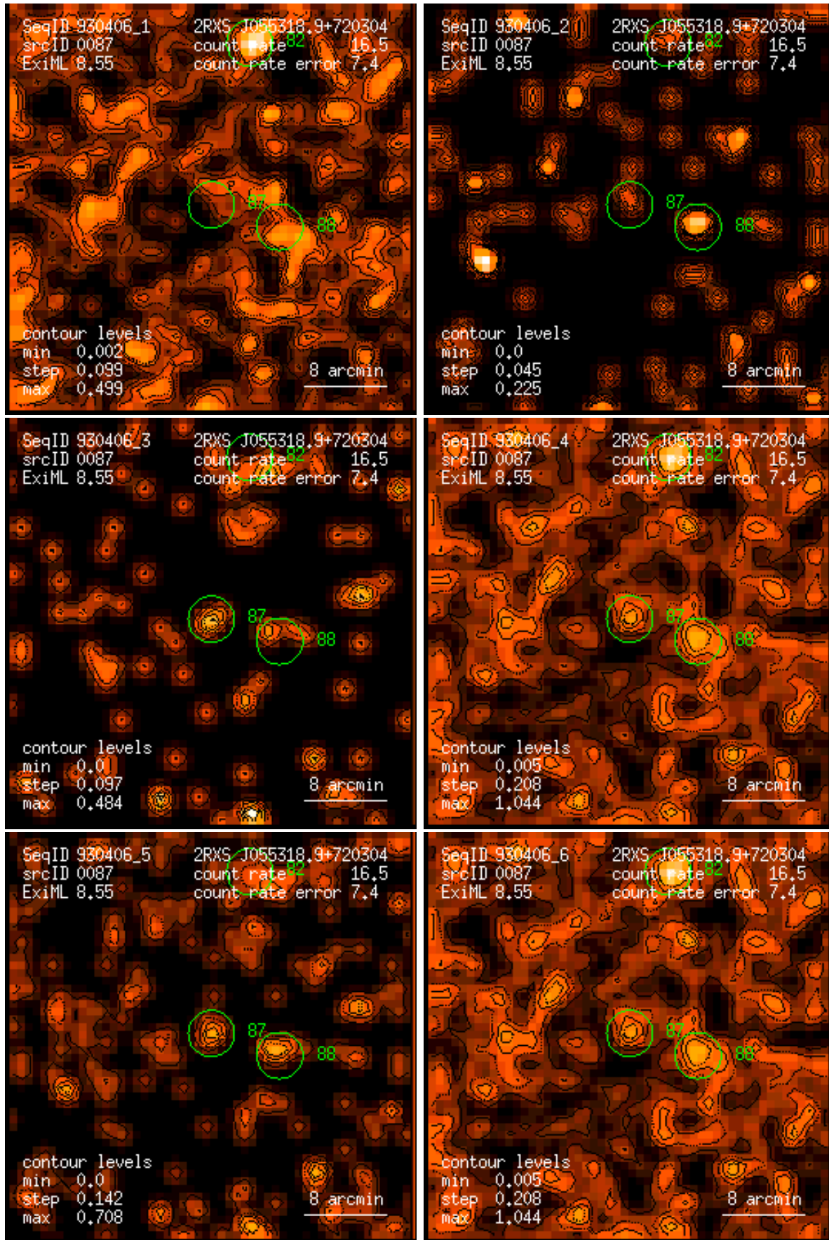
Figure 87: RASS 930406: detection 0087: band rate images, Gaussian filter: (1) PSPC channels 11 – 41, (2) 52 – 90, (3) 91 – 201, (4) 11 – 235, (5) 52 – 201, (6) 11 – 201. Broad band rates in counts/ks. Band rate contour levels in counts/ks/arcmin 2 .
