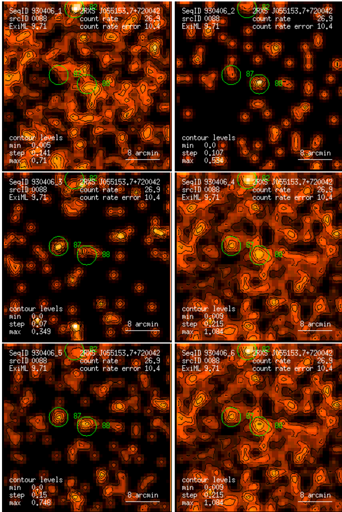
Figure 88: RASS 930406: detection 0088: band rate images, Gaussian filter: (1) PSPC channels 11 – 41, (2) 52 – 90, (3) 91 – 201, (4) 11 – 235, (5) 52 – 201, (6) 11 – 201. Broad band rates in counts/ks. Band rate contour levels in counts/ks/arcmin 2 .
