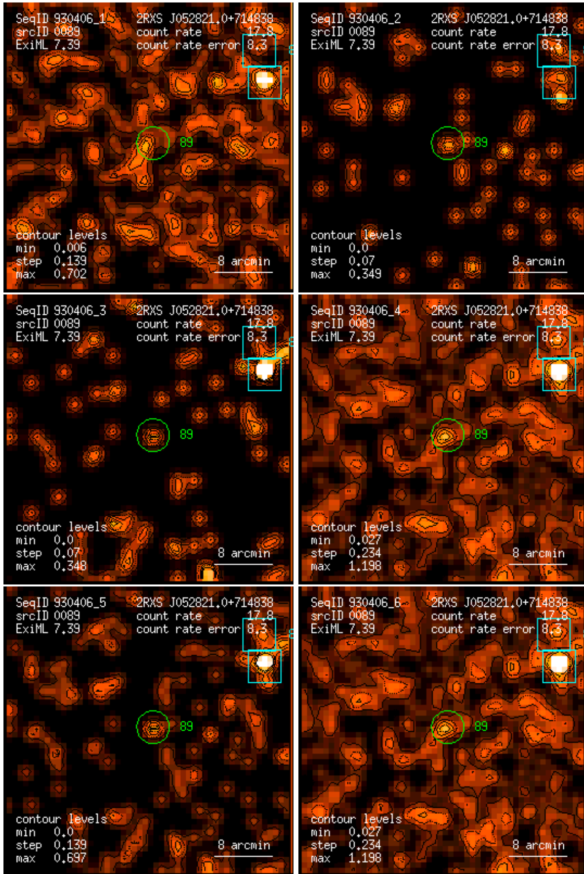
Figure 89: RASS 930406: detection 0089: band rate images, Gaussian filter: (1) PSPC channels 11 – 41, (2) 52 – 90, (3) 91 – 201, (4) 11 – 235, (5) 52 – 201, (6) 11 – 201. Broad band rates in counts/ks. Band rate contour levels in counts/ks/arcmin 2 .
