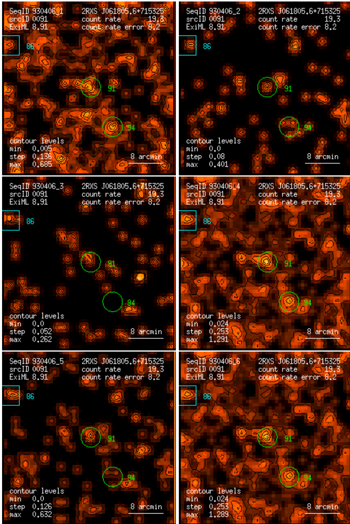
Figure 91: RASS 930406: detection 0091: band rate images, Gaussian filter: (1) PSPC channels 11 – 41, (2) 52 – 90, (3) 91 – 201, (4) 11 – 235, (5) 52 – 201, (6) 11 – 201. Broad band rates in counts/ks. Band rate contour levels in counts/ks/arcmin 2 .
