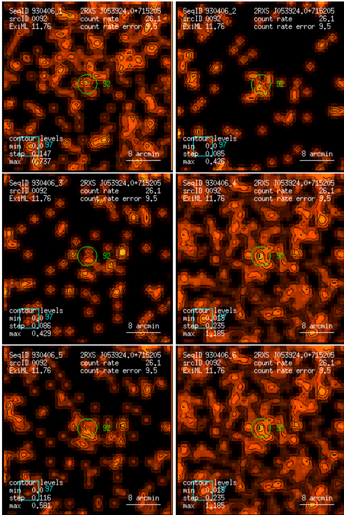
Figure 92: RASS 930406: detection 0092: band rate images, Gaussian filter: (1) PSPC channels 11 – 41, (2) 52 – 90, (3) 91 – 201, (4) 11 – 235, (5) 52 – 201, (6) 11 – 201. Broad band rates in counts/ks. Band rate contour levels in counts/ks/arcmin 2 .
