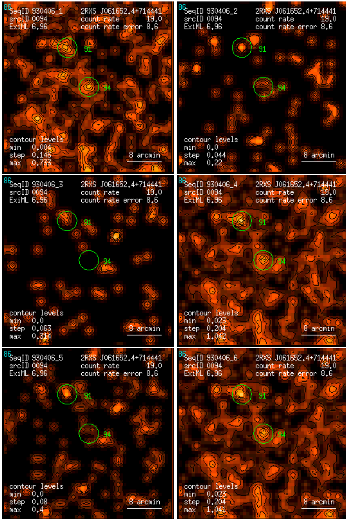
Figure 94: RASS 930406: detection 0094: band rate images, Gaussian filter: (1) PSPC channels 11 – 41, (2) 52 – 90, (3) 91 – 201, (4) 11 – 235, (5) 52 – 201, (6) 11 – 201. Broad band rates in counts/ks. Band rate contour levels in counts/ks/arcmin 2 .
