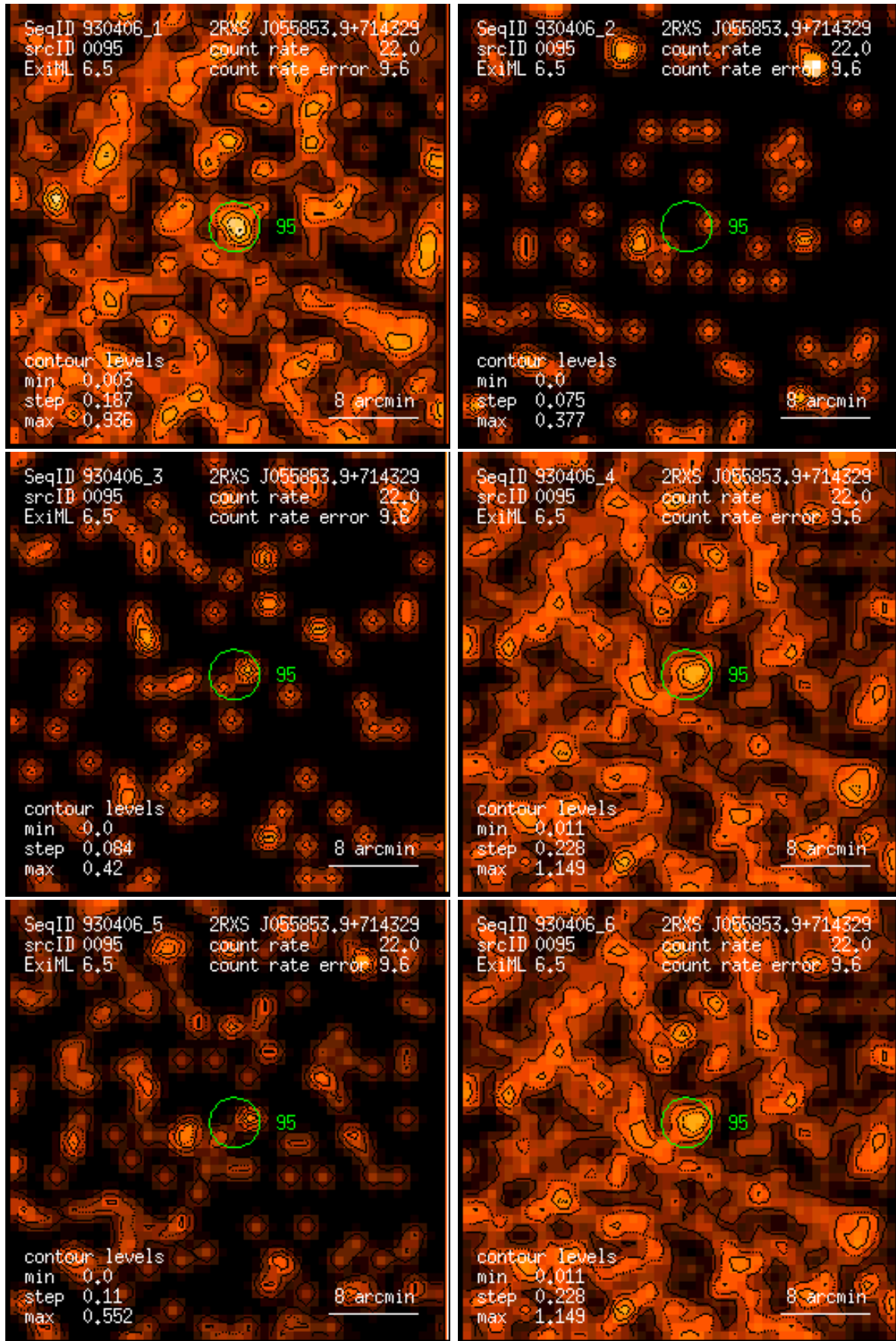
Figure 95: RASS 930406: detection 0095: band rate images, Gaussian filter: (1) PSPC channels 11 – 41, (2) 52 – 90, (3) 91 – 201, (4) 11 – 235, (5) 52 – 201, (6) 11 – 201. Broad band rates in counts/ks. Band rate contour levels in counts/ks/arcmin 2 .
