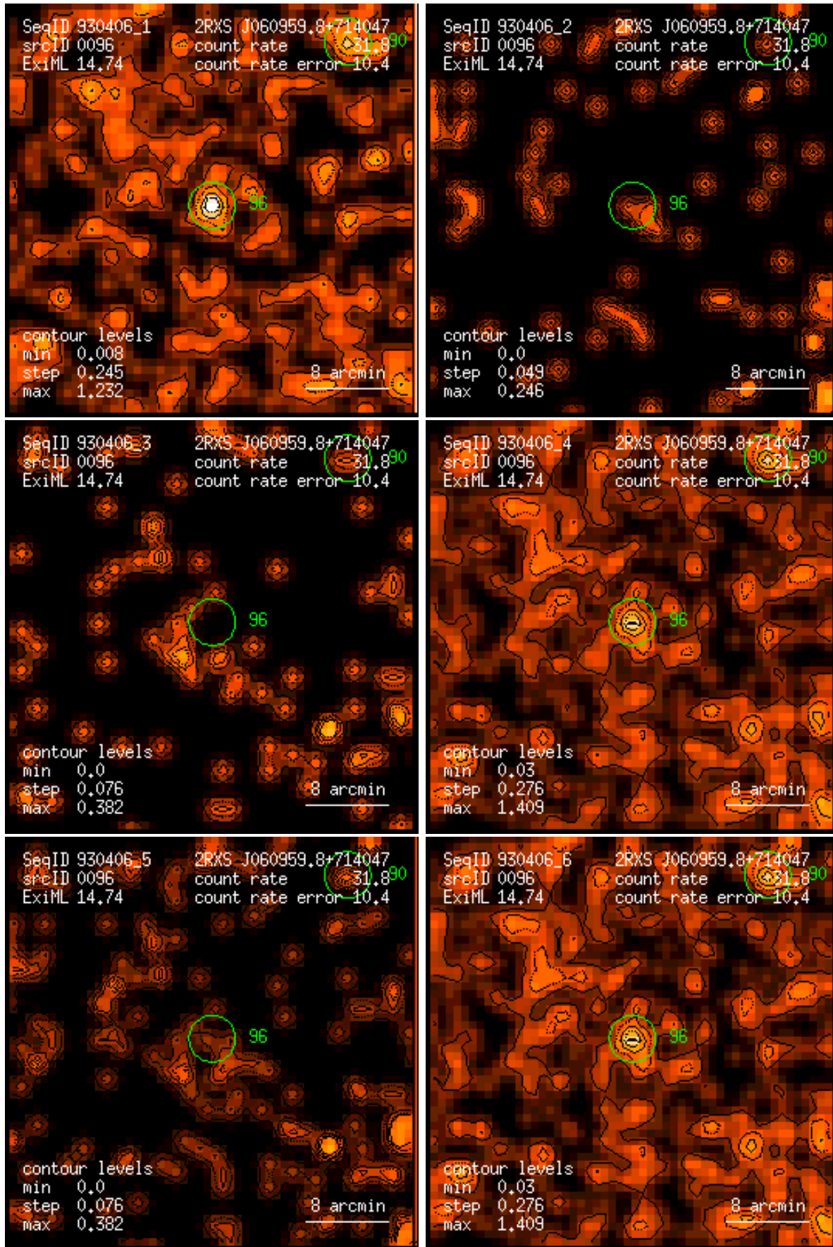
Figure 96: RASS 930406: detection 0096: band rate images, Gaussian filter: (1) PSPC channels 11 – 41, (2) 52 – 90, (3) 91 – 201, (4) 11 – 235, (5) 52 – 201, (6) 11 – 201. Broad band rates in counts/ks. Band rate contour levels in counts/ks/arcmin 2 .
