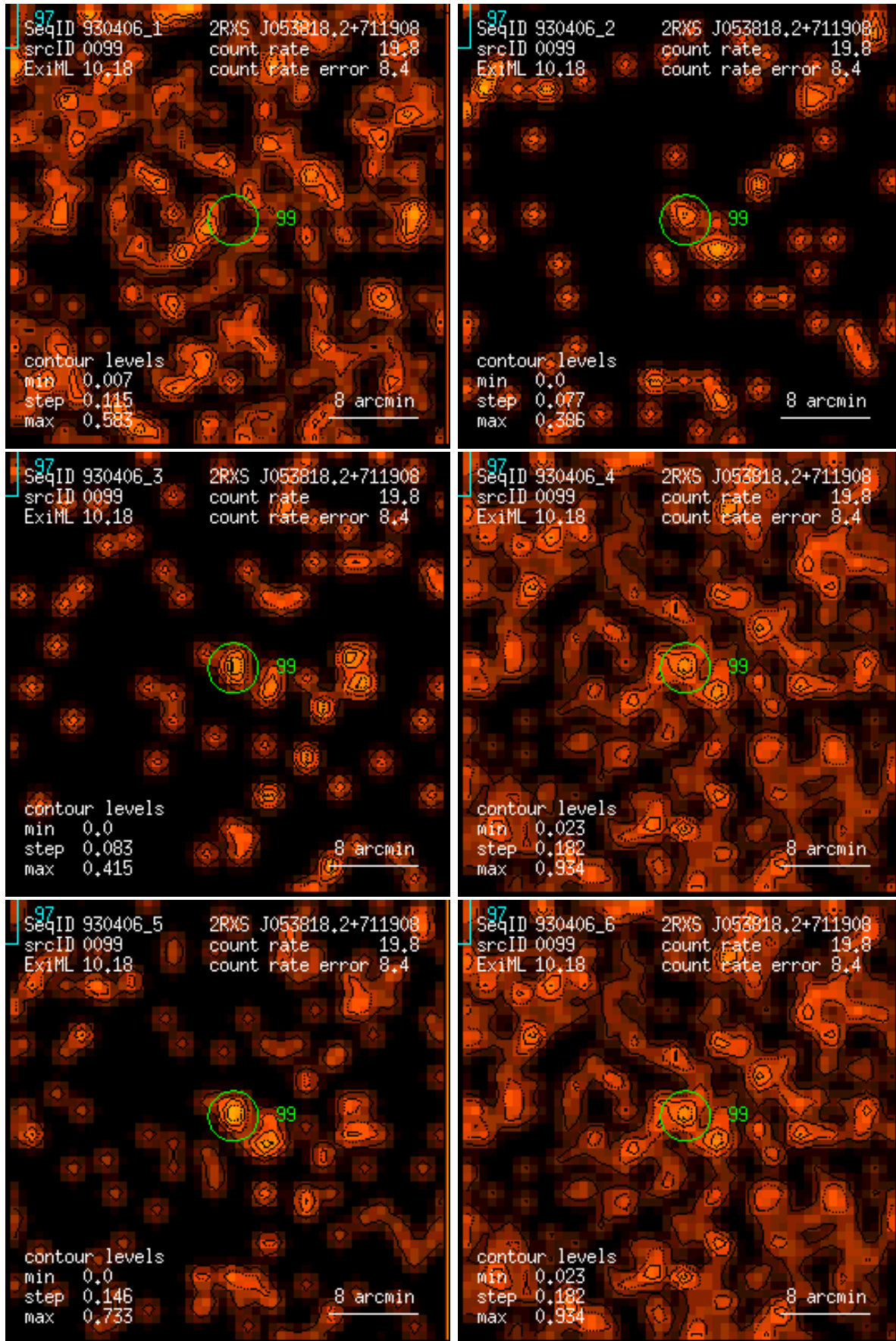
Figure 99: RASS 930406: detection 0099: band rate images, Gaussian filter: (1) PSPC channels 11 – 41, (2) 52 – 90, (3) 91 – 201, (4) 11 – 235, (5) 52 – 201, (6) 11 – 201. Broad band rates in counts/ks. Band rate contour levels in counts/ks/arcmin 2 .
