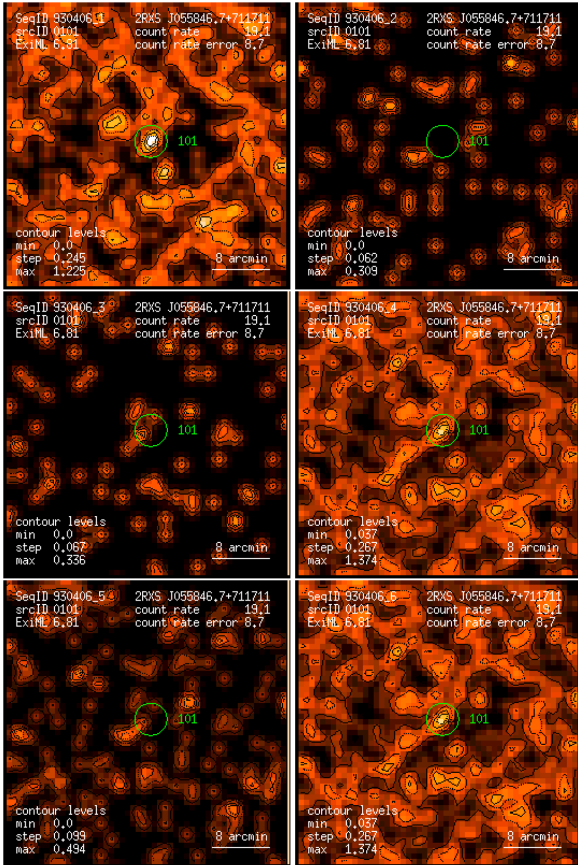
Figure 101: RASS 930406: detection 0101: band rate images, Gaussian filter: (1) PSPC channels 11 – 41, (2) 52 – 90, (3) 91 – 201, (4) 11 – 235, (5) 52 – 201, (6) 11 – 201. Broad band rates in counts/ks. Band rate contour levels in counts/ks/arcmin 2 .
