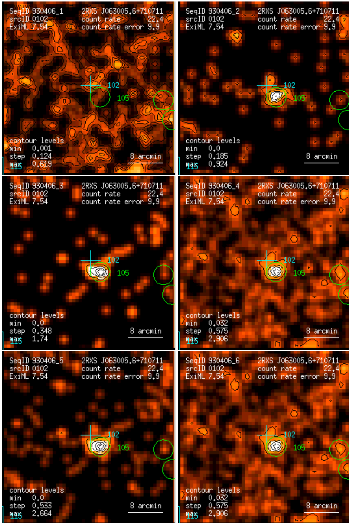
Figure 102: RASS 930406: detection 0102: band rate images, Gaussian filter: (1) PSPC channels 11 – 41, (2) 52 – 90, (3) 91 – 201, (4) 11 – 235, (5) 52 – 201, (6) 11 – 201. Broad band rates in counts/ks. Band rate contour levels in counts/ks/arcmin 2 .
