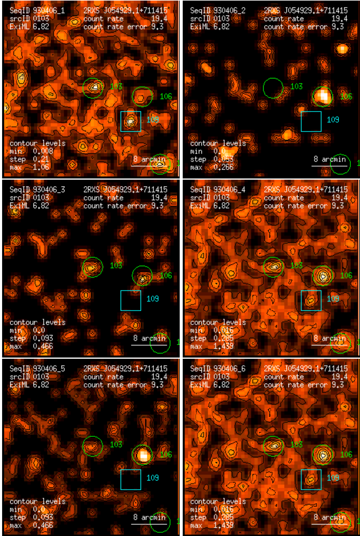
Figure 103: RASS 930406: detection 0103: band rate images, Gaussian filter: (1) PSPC channels 11 – 41, (2) 52 – 90, (3) 91 – 201, (4) 11 – 235, (5) 52 – 201, (6) 11 – 201. Broad band rates in counts/ks. Band rate contour levels in counts/ks/arcmin 2 .
