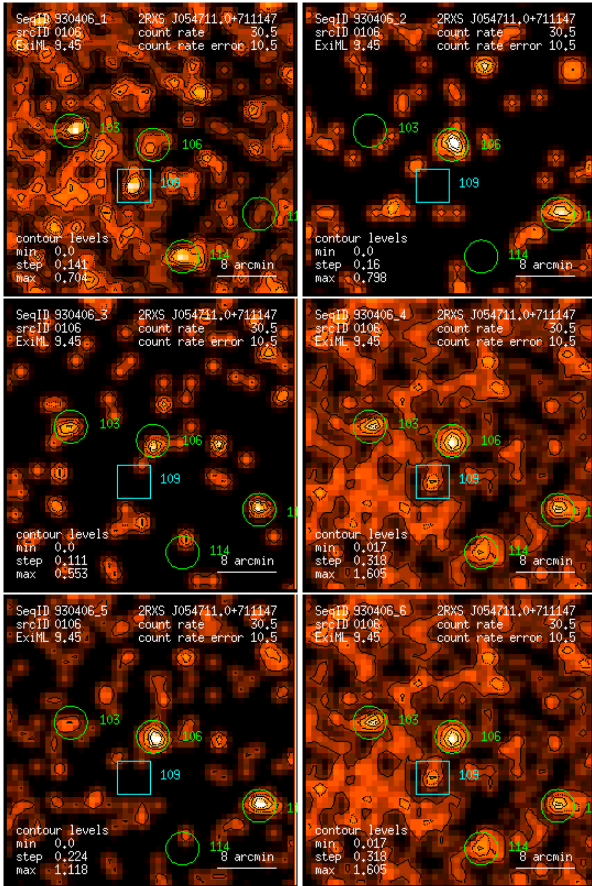
Figure 106: RASS 930406: detection 0106: band rate images, Gaussian filter: (1) PSPC channels 11 – 41, (2) 52 – 90, (3) 91 – 201, (4) 11 – 235, (5) 52 – 201, (6) 11 – 201. Broad band rates in counts/ks. Band rate contour levels in counts/ks/arcmin 2 .
