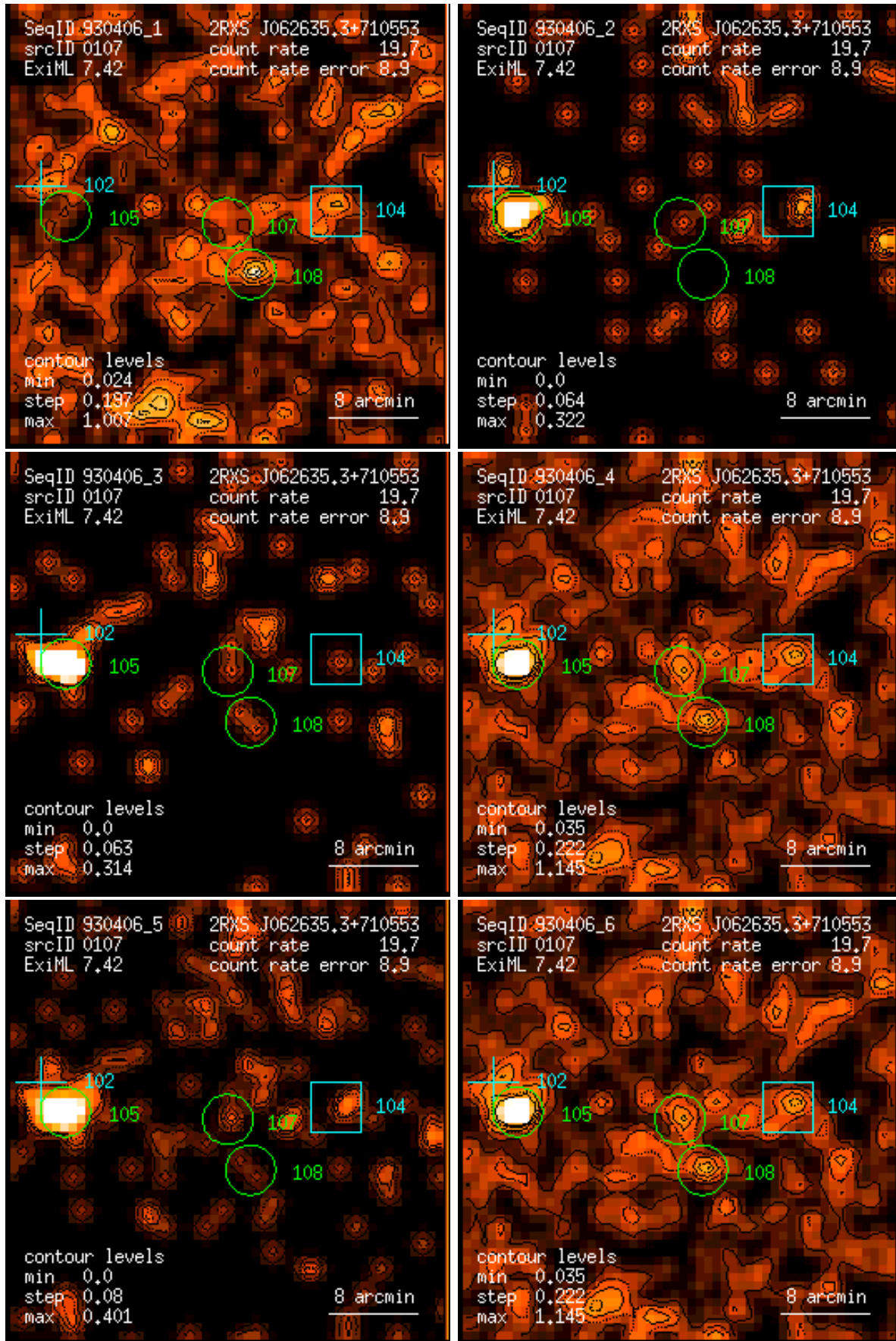
Figure 107: RASS 930406: detection 0107: band rate images, Gaussian filter: (1) PSPC channels 11 – 41, (2) 52 – 90, (3) 91 – 201, (4) 11 – 235, (5) 52 – 201, (6) 11 – 201. Broad band rates in counts/ks. Band rate contour levels in counts/ks/arcmin 2 .
