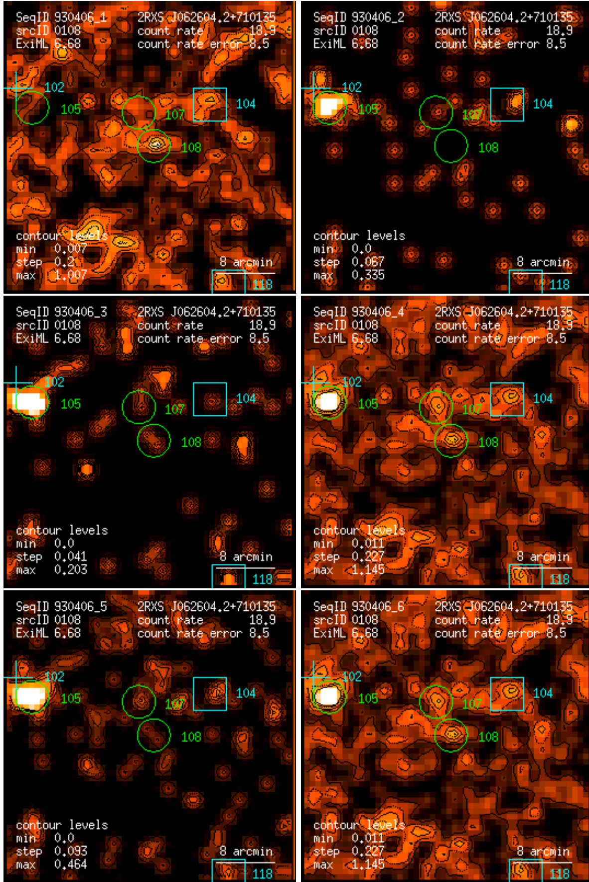
Figure 108: RASS 930406: detection 0108: band rate images, Gaussian filter: (1) PSPC channels 11 – 41, (2) 52 – 90, (3) 91 – 201, (4) 11 – 235, (5) 52 – 201, (6) 11 – 201. Broad band rates in counts/ks. Band rate contour levels in counts/ks/arcmin 2 .
