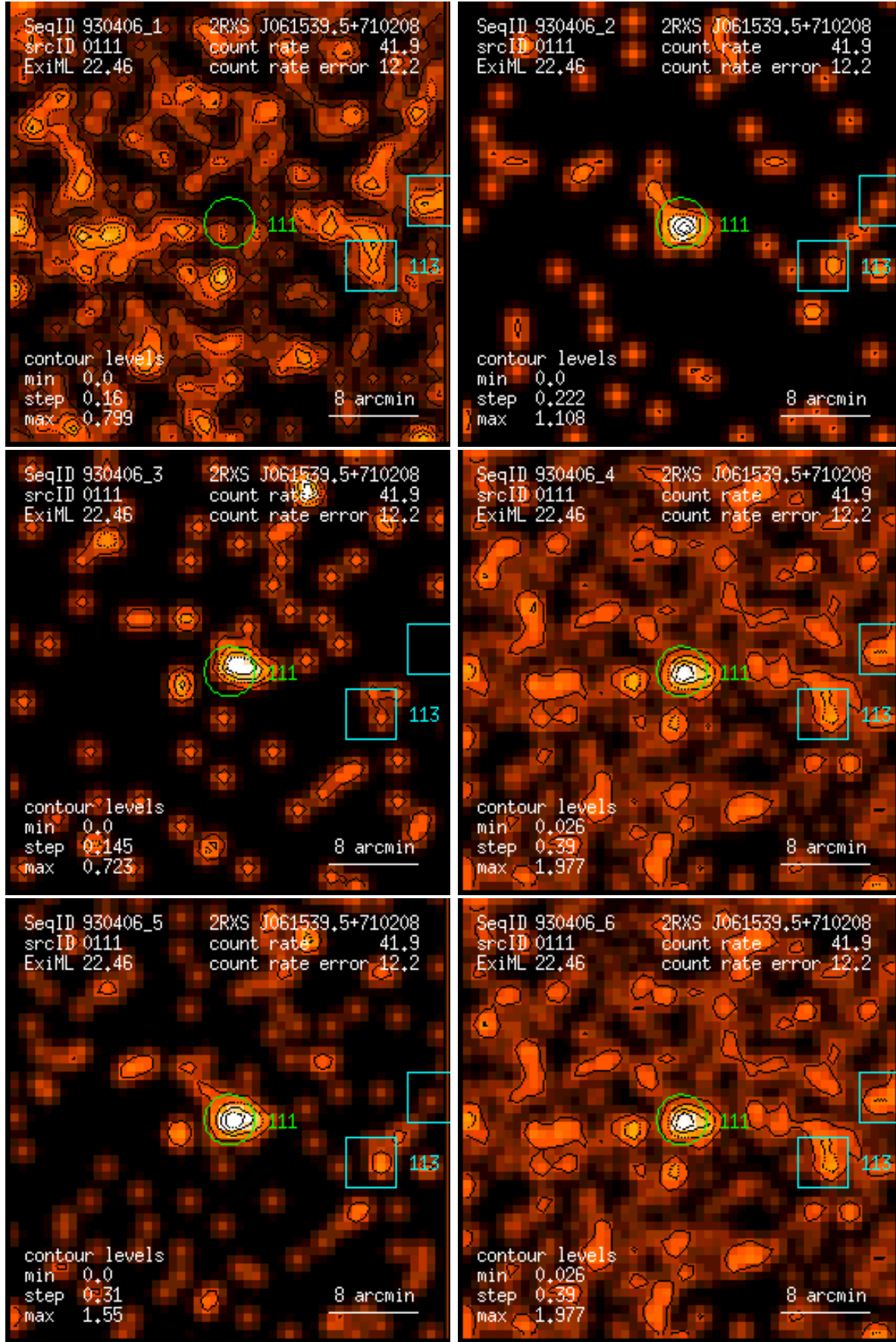
Figure 111: RASS 930406: detection 0111: band rate images, Gaussian filter: (1) PSPC channels 11 – 41, (2) 52 – 90, (3) 91 – 201, (4) 11 – 235, (5) 52 – 201, (6) 11 – 201. Broad band rates in counts/ks. Band rate contour levels in counts/ks/arcmin 2 .
