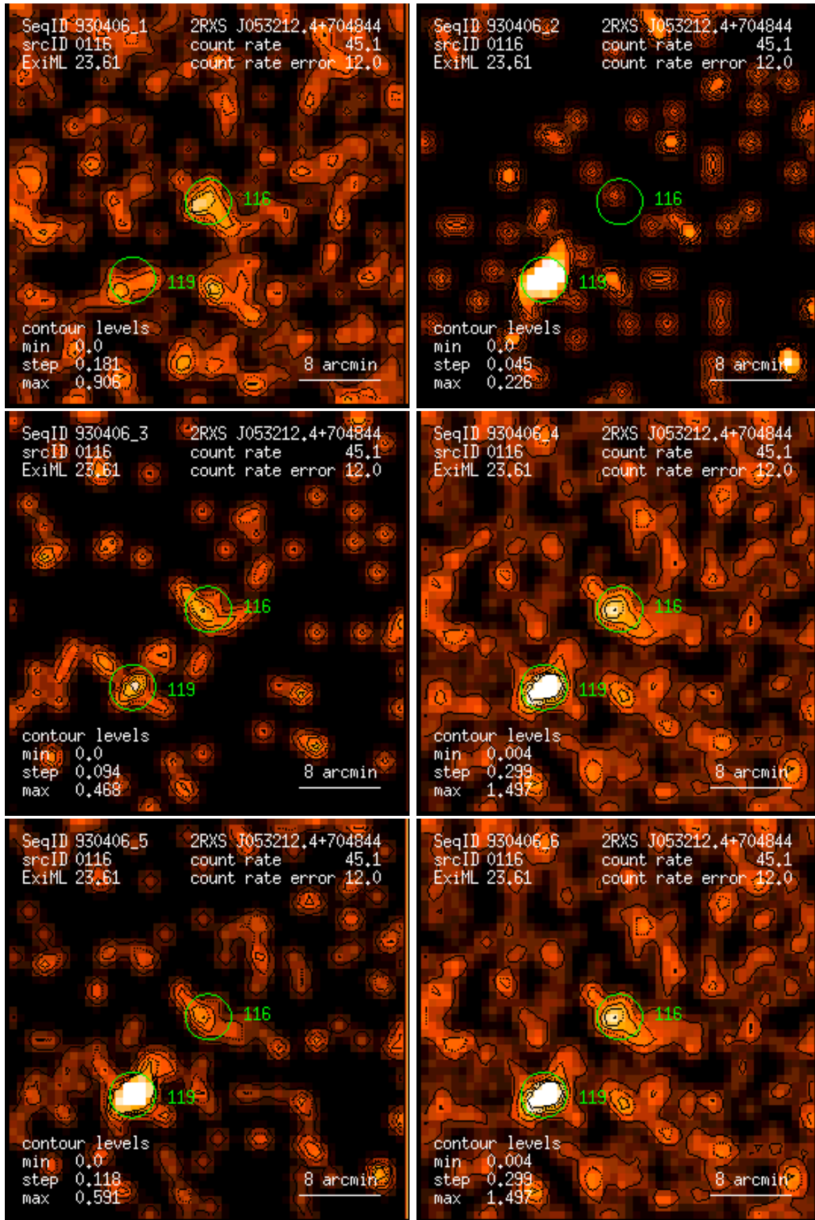
Figure 116: RASS 930406: detection 0116: band rate images, Gaussian filter: (1) PSPC channels 11 – 41, (2) 52 – 90, (3) 91 – 201, (4) 11 – 235, (5) 52 – 201, (6) 11 – 201. Broad band rates in counts/ks. Band rate contour levels in counts/ks/arcmin 2 .
