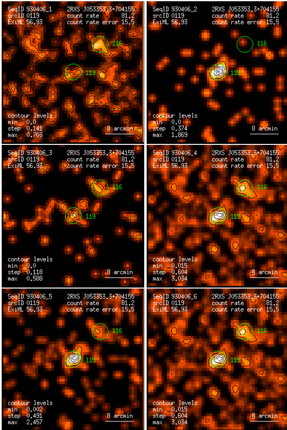
Figure 119: RASS 930406: detection 0119: band rate images, Gaussian filter: (1) PSPC channels 11 – 41, (2) 52 – 90, (3) 91 – 201, (4) 11 – 235, (5) 52 – 201, (6) 11 – 201. Broad band rates in counts/ks. Band rate contour levels in counts/ks/arcmin 2 .
