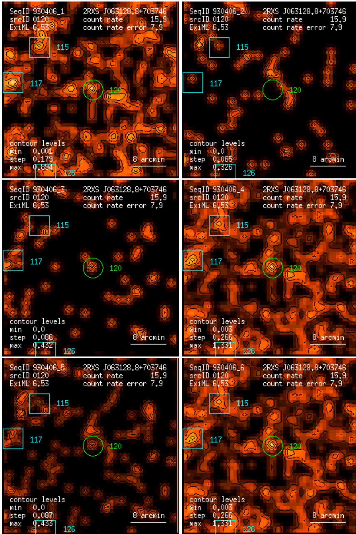
Figure 120: RASS 930406: detection 0120: band rate images, Gaussian filter: (1) PSPC channels 11 – 41, (2) 52 – 90, (3) 91 – 201, (4) 11 – 235, (5) 52 – 201, (6) 11 – 201. Broad band rates in counts/ks. Band rate contour levels in counts/ks/arcmin 2 .
