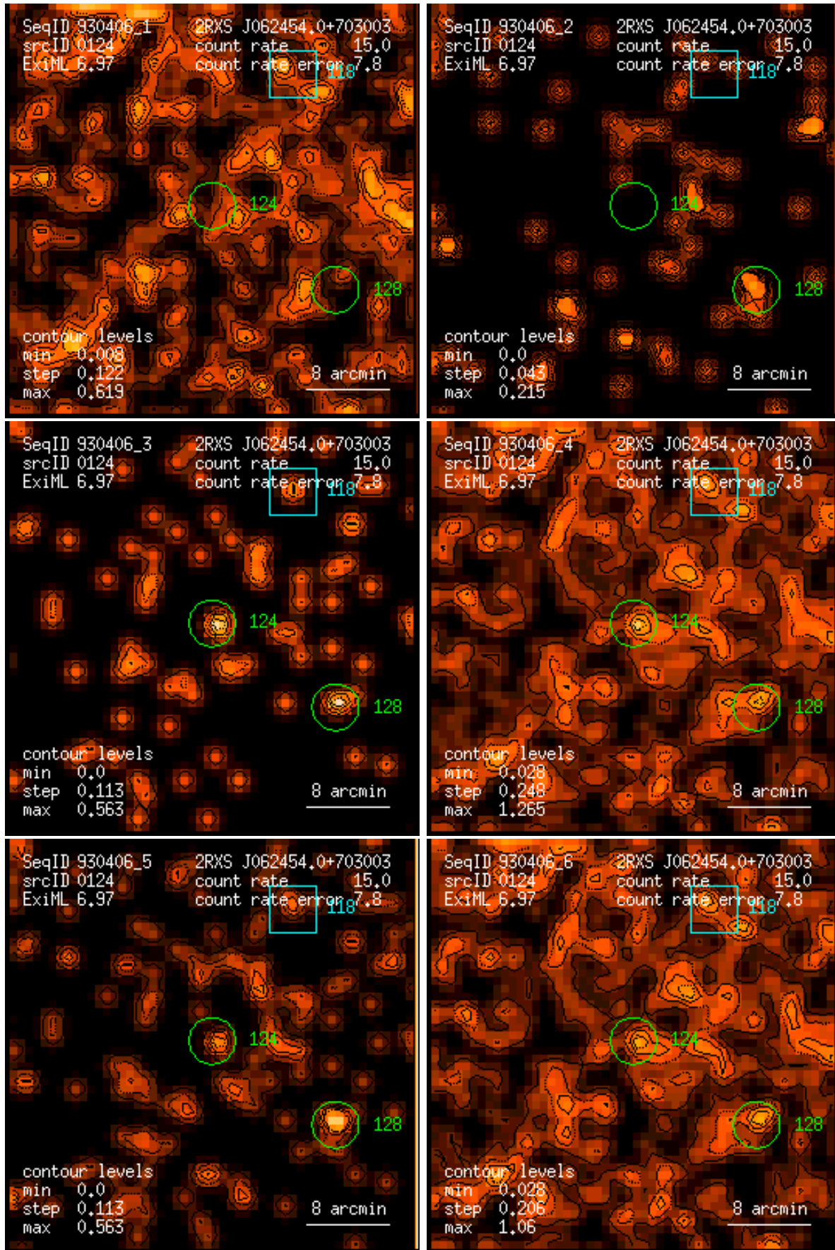
Figure 124: RASS 930406: detection 0124: band rate images, Gaussian filter: (1) PSPC channels 11 – 41, (2) 52 – 90, (3) 91 – 201, (4) 11 – 235, (5) 52 – 201, (6) 11 – 201. Broad band rates in counts/ks. Band rate contour levels in counts/ks/arcmin 2 .
