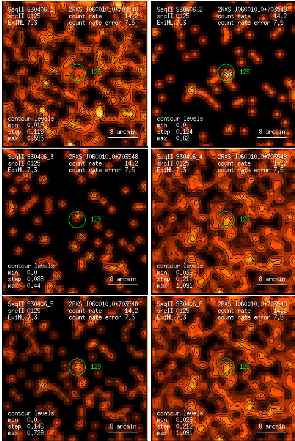
Figure 125: RASS 930406: detection 0125: band rate images, Gaussian filter: (1) PSPC channels 11 – 41, (2) 52 – 90, (3) 91 – 201, (4) 11 – 235, (5) 52 – 201, (6) 11 – 201. Broad band rates in counts/ks. Band rate contour levels in counts/ks/arcmin 2 .
