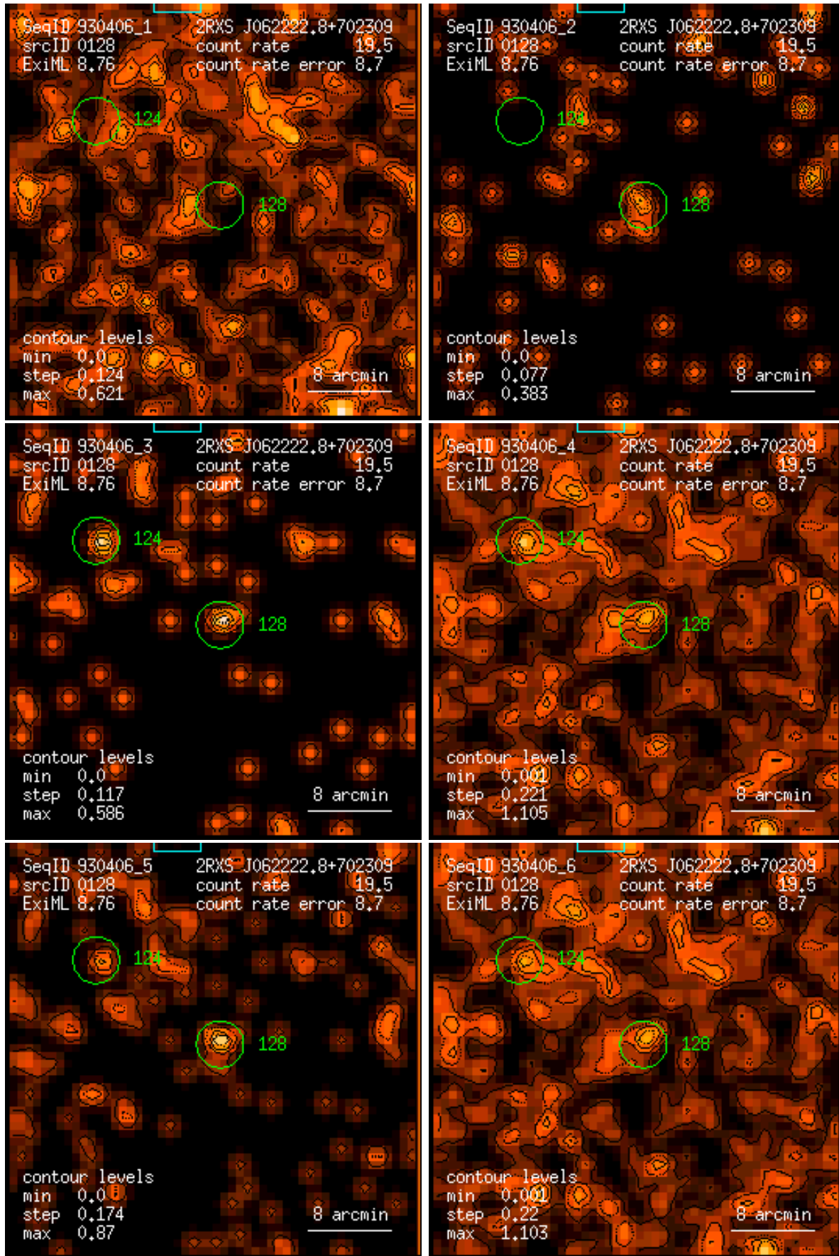
Figure 128: RASS 930406: detection 0128: band rate images, Gaussian filter: (1) PSPC channels 11 – 41, (2) 52 – 90, (3) 91 – 201, (4) 11 – 235, (5) 52 – 201, (6) 11 – 201. Broad band rates in counts/ks. Band rate contour levels in counts/ks/arcmin 2 .
